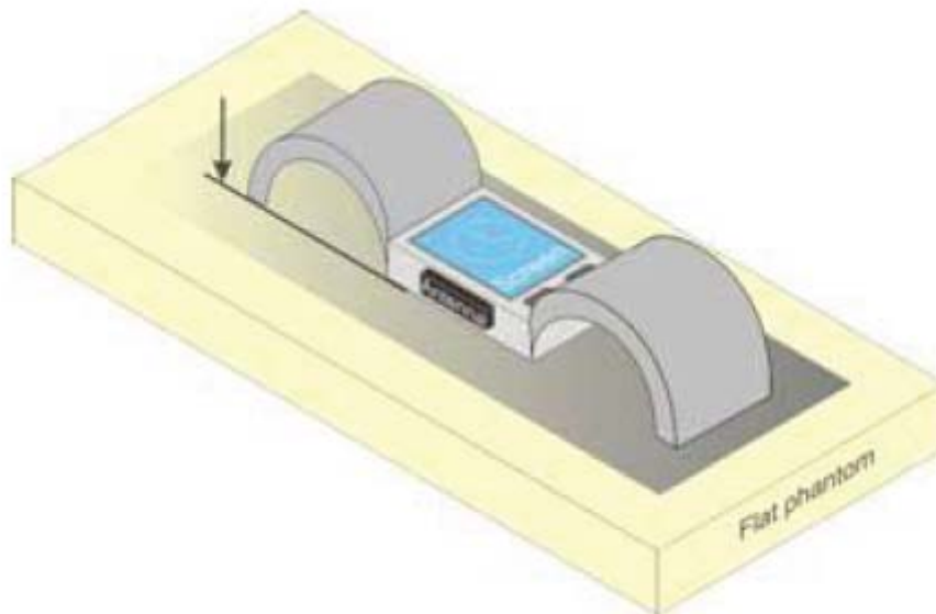
Figure 10 – Test position for limb-worn devices
