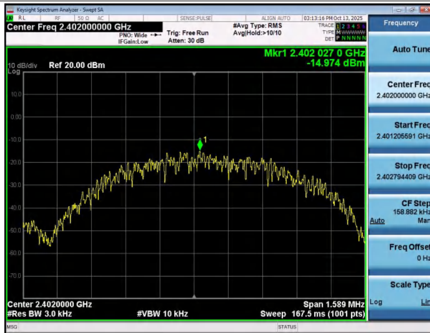
Power_Spectral_Density_BLE_1Mbps_2402
