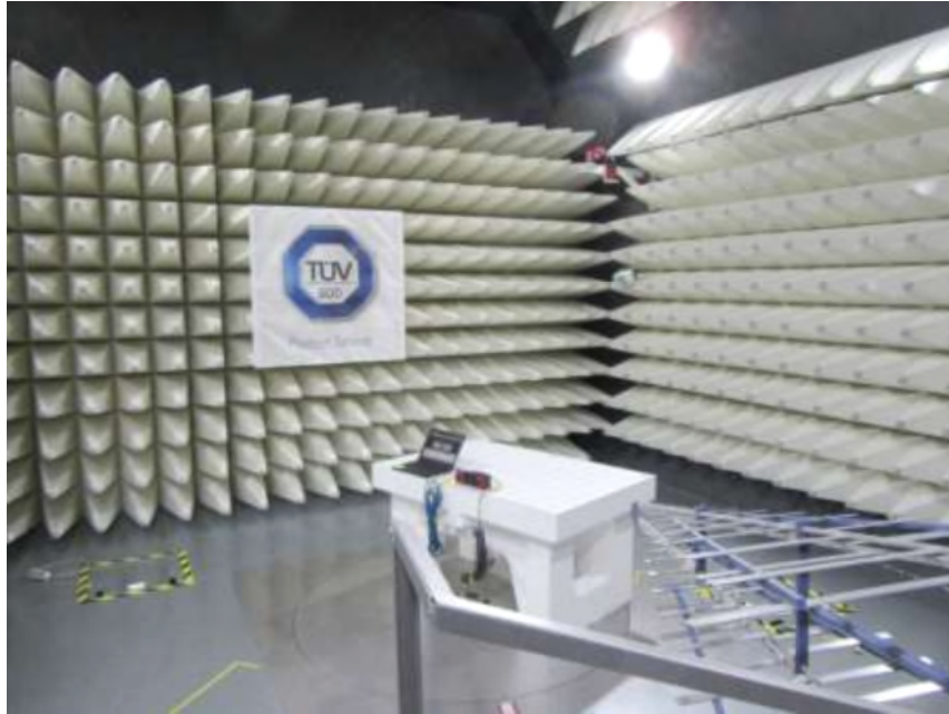
Figure 1 - Radiated emissions
