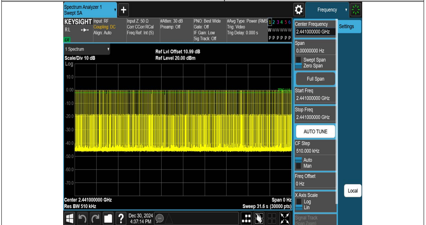
3DH1-Ant1-Hop-PASS
