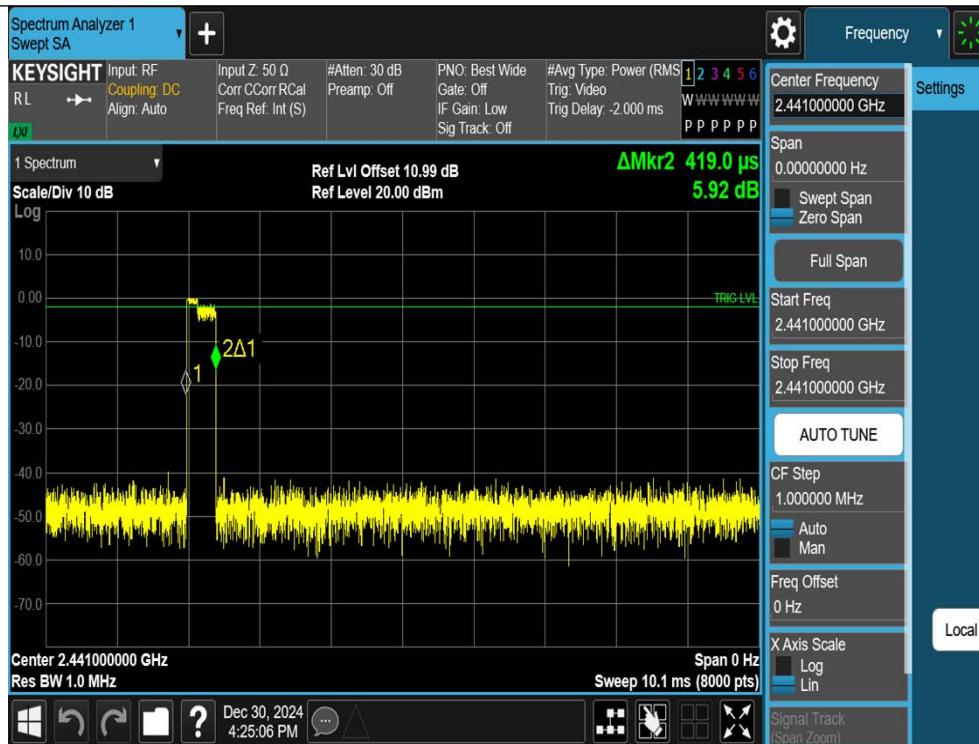
2DH1-Ant1-Hop-PASS
