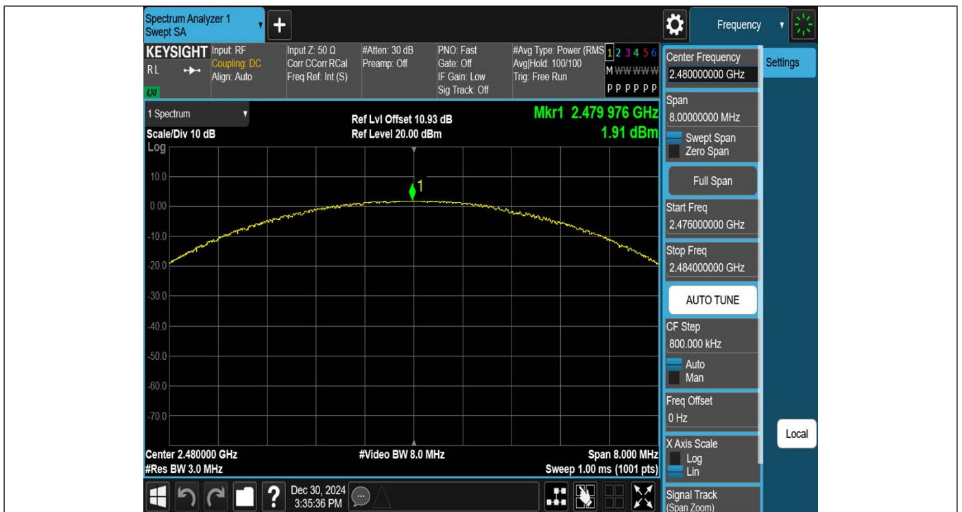
2DH5-Ant1-2480-PASS
