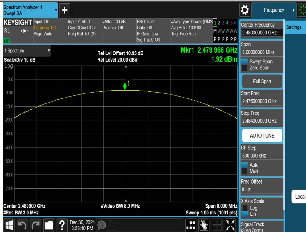
DH5-Ant1-2480-PASS
