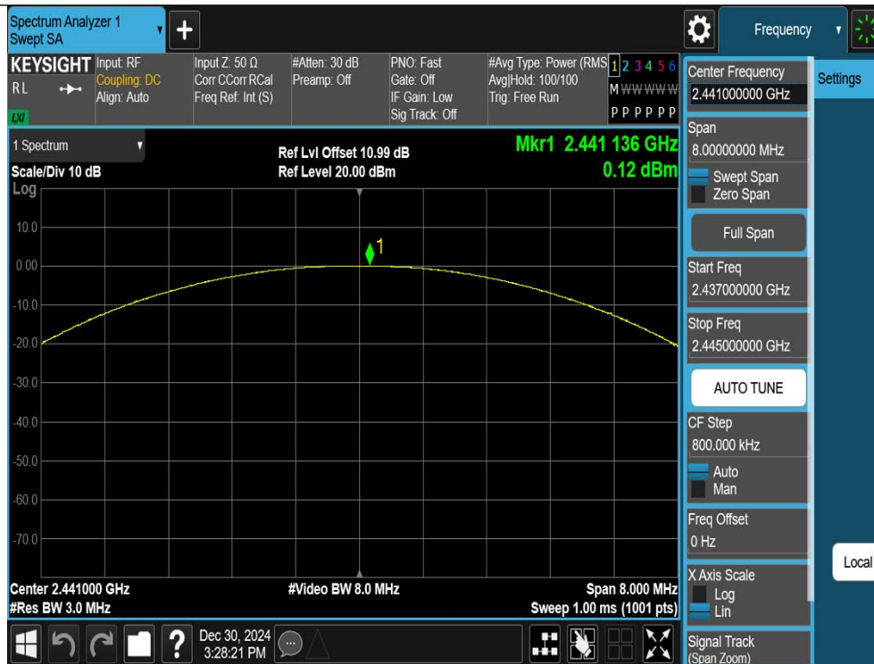
DH5-Ant1-2441-PASS
