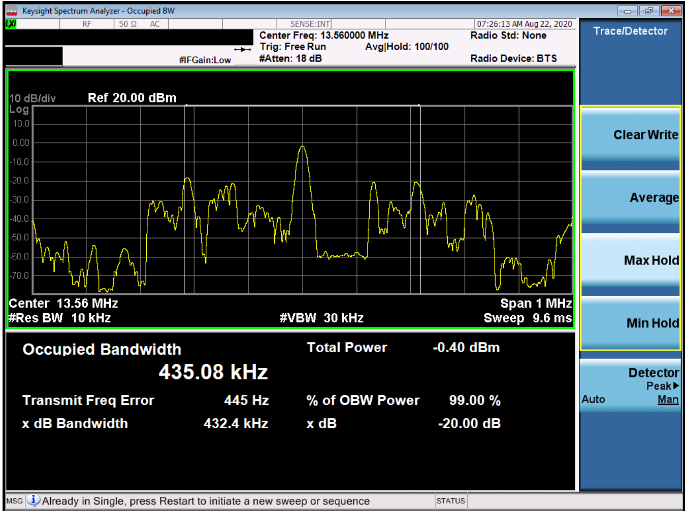
Figure 7-3. Occupied Bandwidth Plot MIT22
