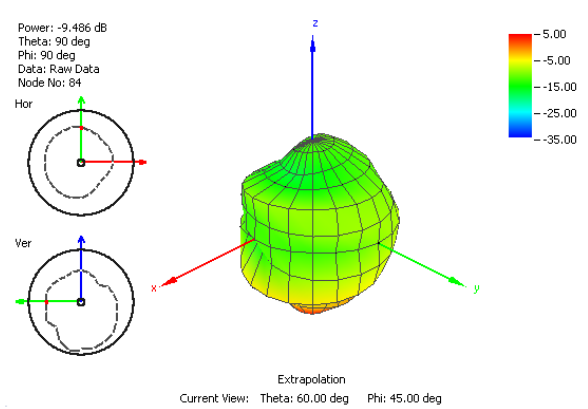
Figure 19. Radiation Pattern at 849MHz of G30 Antenna in Free Space
