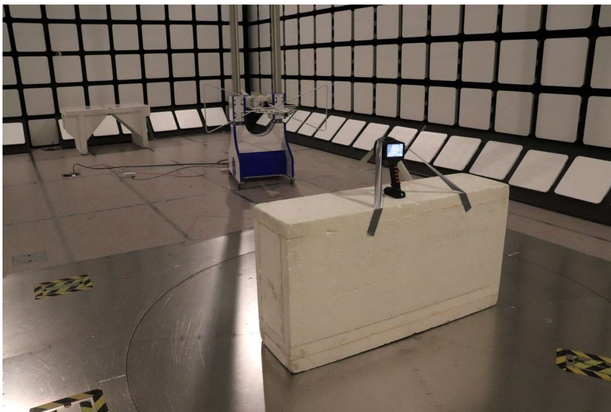
Photograph 4. Radiated Emissions 30 – 1000 MHz
