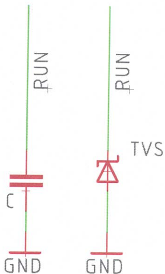
The schematics of the signal protection components of the run signal.
