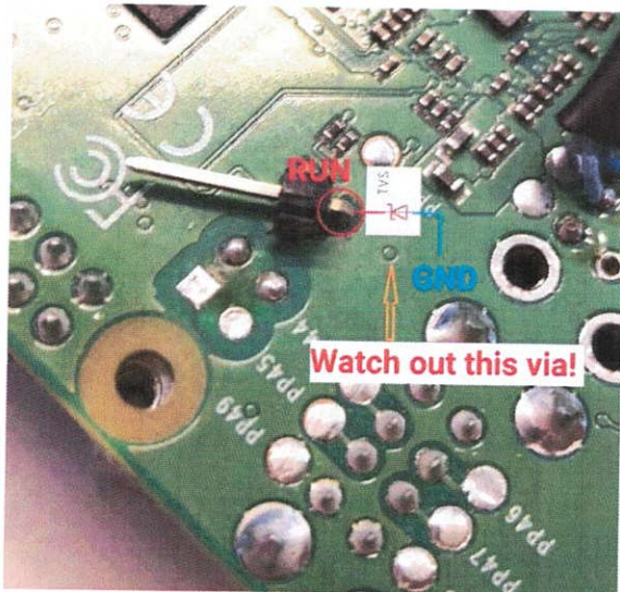
The placement of the TVS diode nearby the pin header
