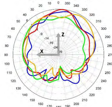
Side to Side XZ 3700 MHz
