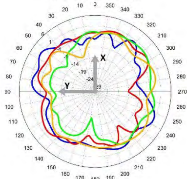
Azimuth XY 3700 MHz
