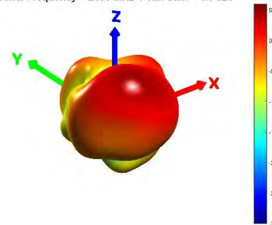
Cell4: Frequency = 2100 MHz Peak Gain = 4.6 dBi
