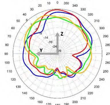
Front to Back YZ 3700 MHz
