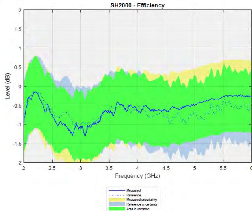
Figure 5.62: Efficiency
