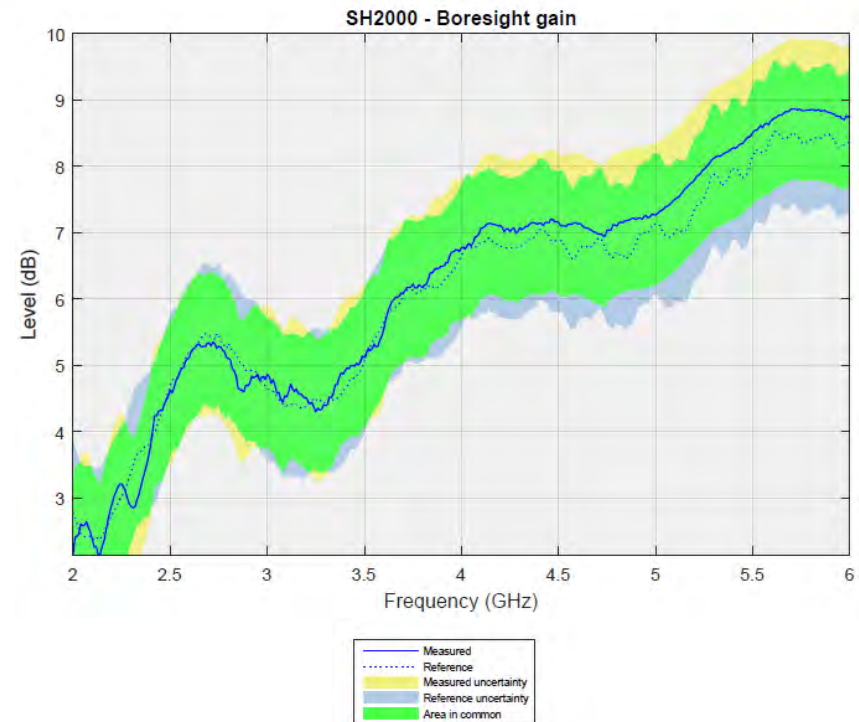
Figure 5.61: Boresight gain
