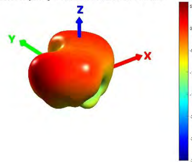
Cell3: Frequency = 1800 MHz Peak Gain = 2.7 dBi
