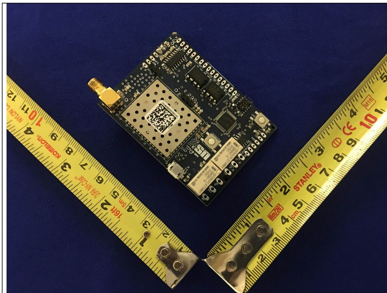
EUT Main Board Top View
