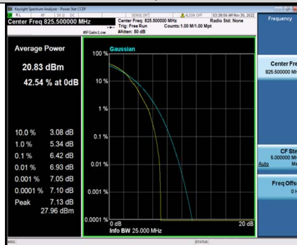
Band26-3MHz-64QAM-26805-15RB#0
