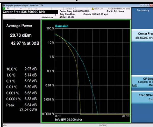
Band26-3MHz-16QAM-27025-1RB#0
