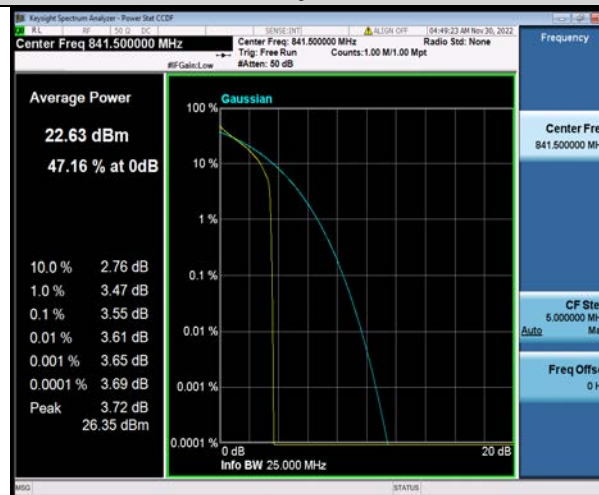
Band26-15MHz-QPSK-26965-75RB#0
