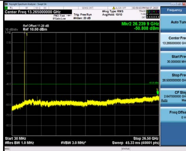
Band30-5MHz-QPSK-27735-1RB#0-Range1:30~26500MHz
