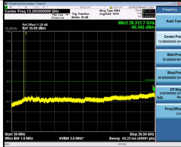
Band30-5MHz-QPSK-27710-1RB#0-Range1:30~26500MHz
