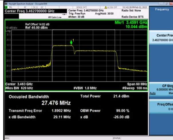
42-42-10MHz-20MHz-QPSK-QPSK-42496-42640-50RB#0-100RB#0
