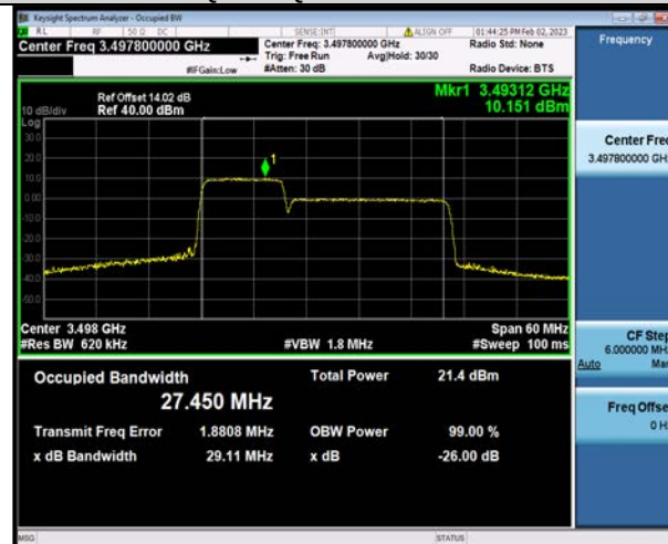
42-42-10MHz-20MHz-QPSK-QPSK-42846-42990-50RB#0-100RB#0
