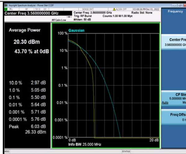
Band48-20MHz-16QAM-55340-100RB#0
