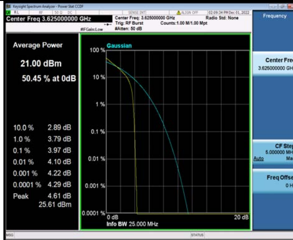
Band48-5MHz-QPSK-55990-25RB#0
