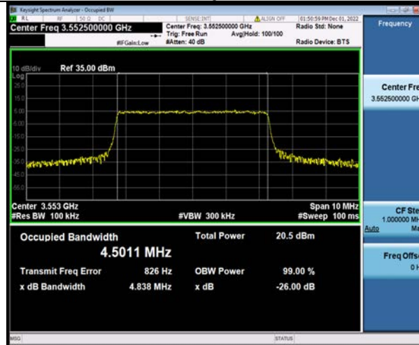
Band48-5MHz-64QAM-55990-25RB#0
