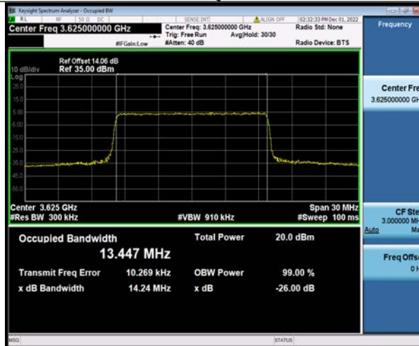
Band48-15MHz-16QAM-56665-75RB#0
