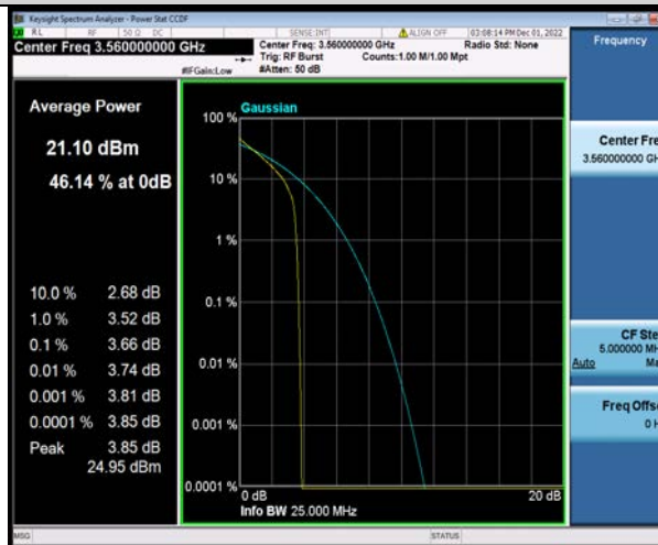
Band48-20MHz-QPSK-55340-100RB#0
