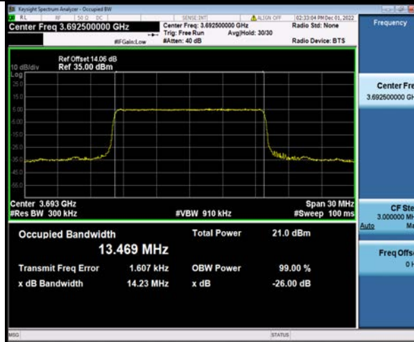
Band48-15MHz-16QAM-55315-75RB#0
