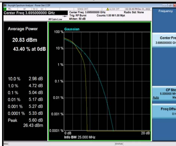
Band48-10MHz-16QAM-56690-50RB#0
