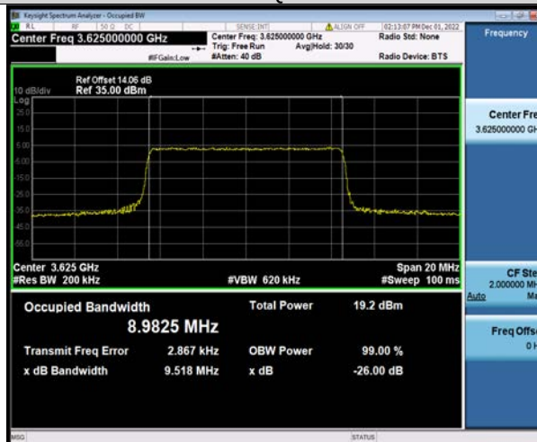
Band48-10MHz-64QAM-56690-50RB#0
