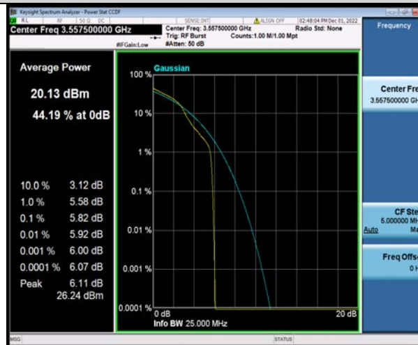
Band48-15MHz-16QAM-55315-75RB#0
