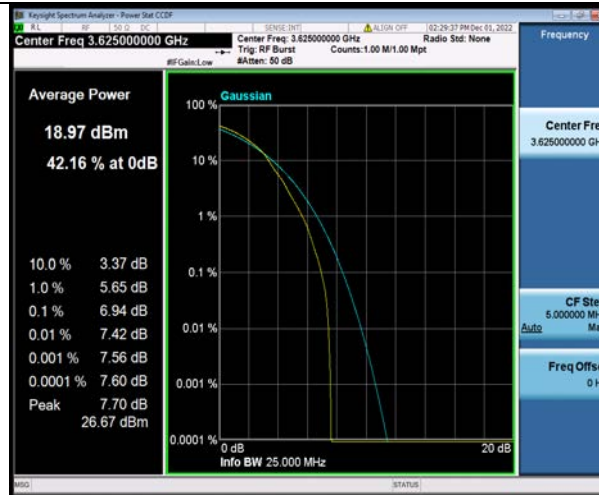
Band48-10MHz-64QAM-55990-50RB#0
