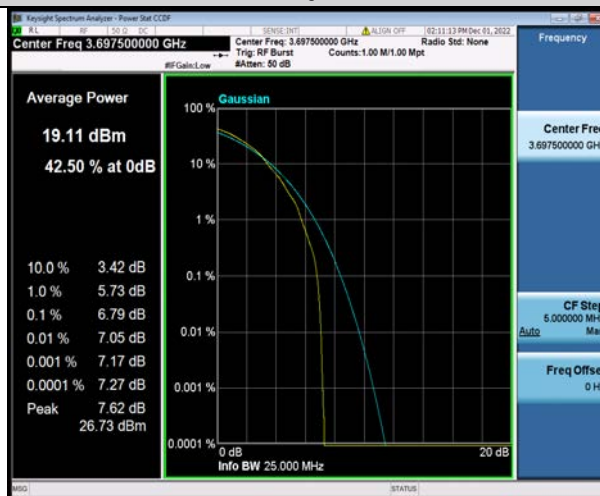
Band48-5MHz-64QAM-56715-25RB#0
