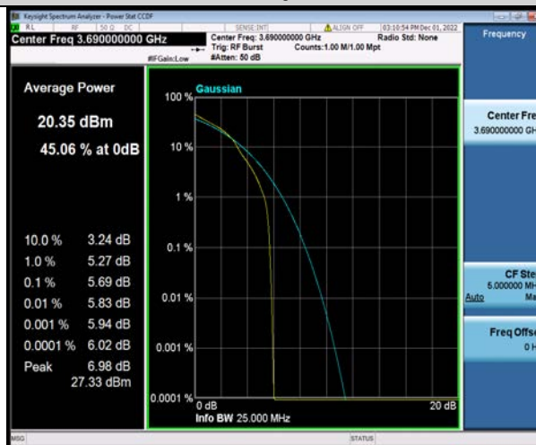
Band48-20MHz-16QAM-56640-100RB#0
