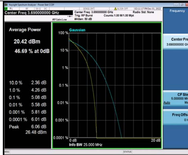
Band48-20MHz-16QAM-55340-1RB#0
