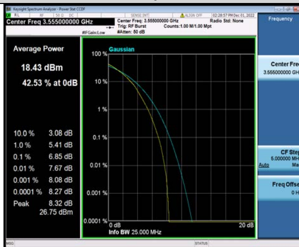
Band48-10MHz-64QAM-55990-1RB#0
