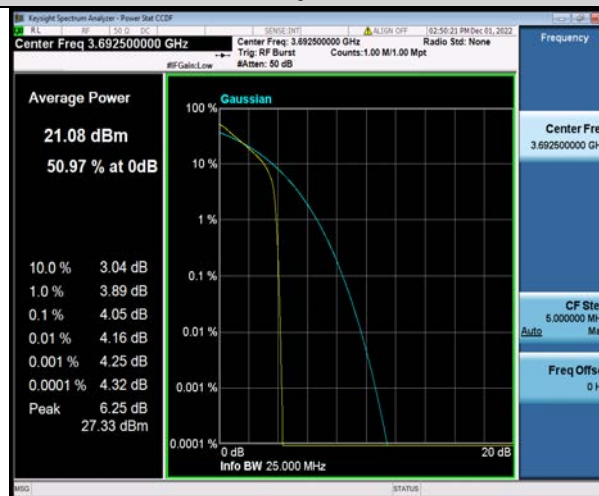
Band48-15MHz-QPSK-56665-75RB#0
