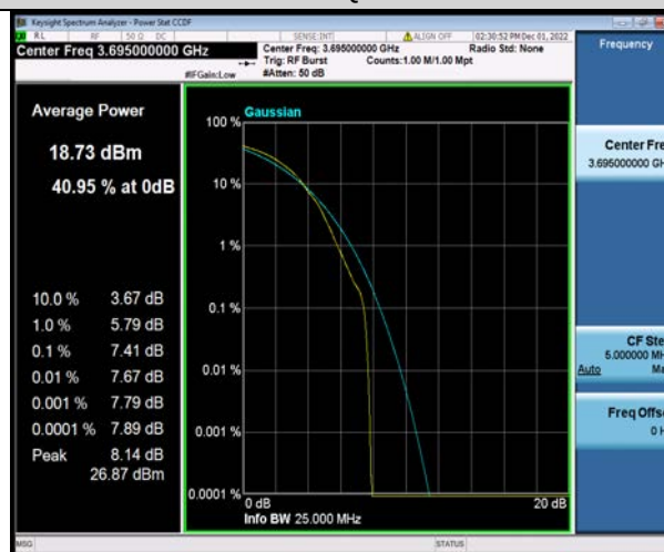
Band48-10MHz-64QAM-56690-50RB#0
