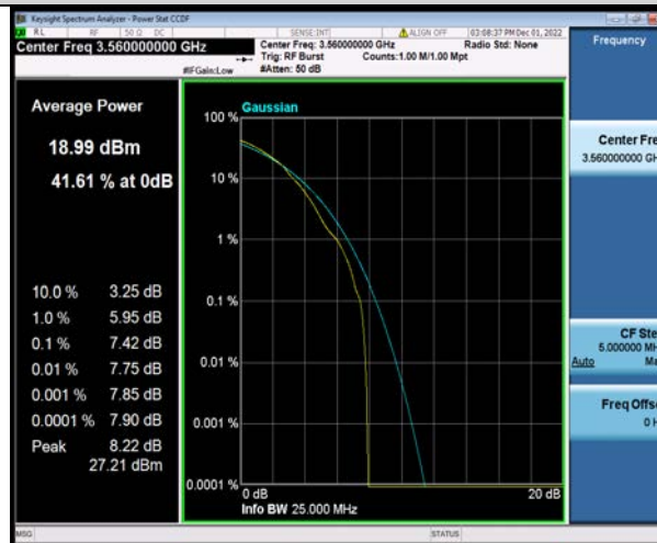
Band48-20MHz-64QAM-55340-100RB#0
