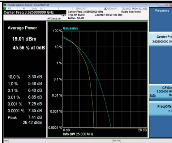
Band48-5MHz-16QAM-56715-1RB#0
