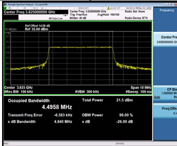
Band48-5MHz-16QAM-56715-25RB#0
