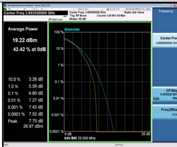
Band48-15MHz-64QAM-56665-75RB#0
