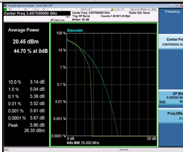
Band48-5MHz-16QAM-56715-25RB#0
