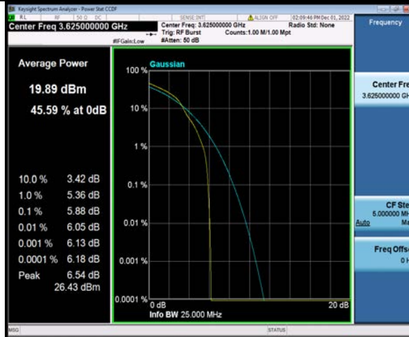
Band48-5MHz-16QAM-55990-25RB#0
