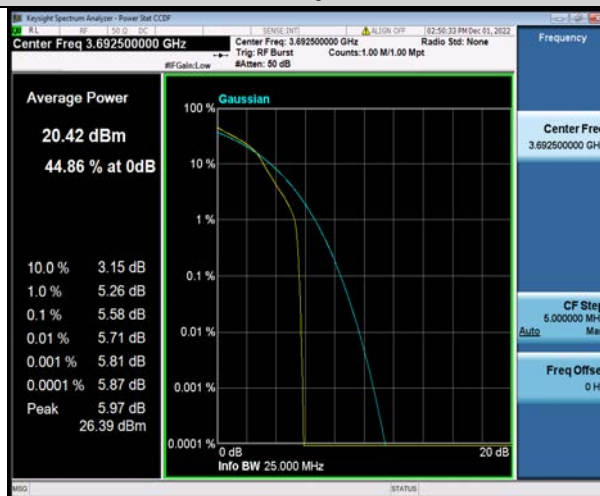
Band48-15MHz-16QAM-56665-75RB#0
