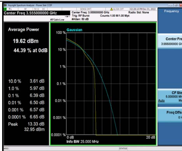
Band48-10MHz-16QAM-55290-50RB#0
