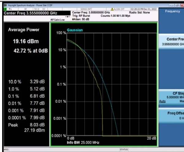
Band48-10MHz-64QAM-55290-50RB#0
