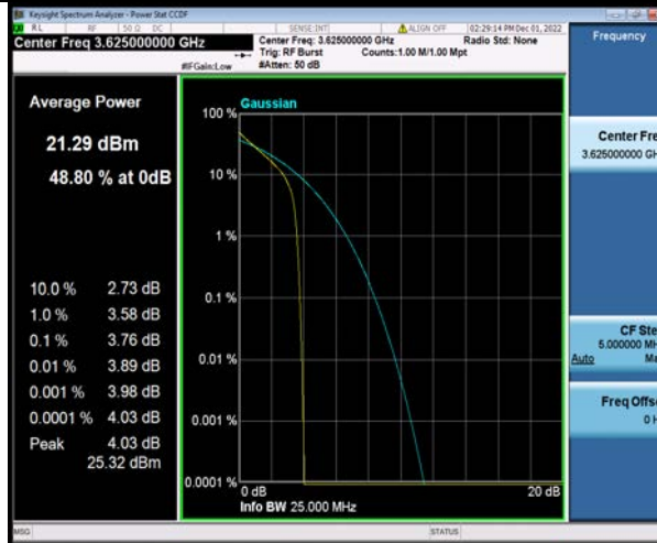
Band48-10MHz-QPSK-55990-50RB#0
