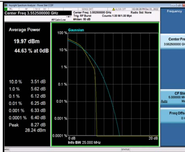
Band48-5MHz-16QAM-55265-25RB#0
