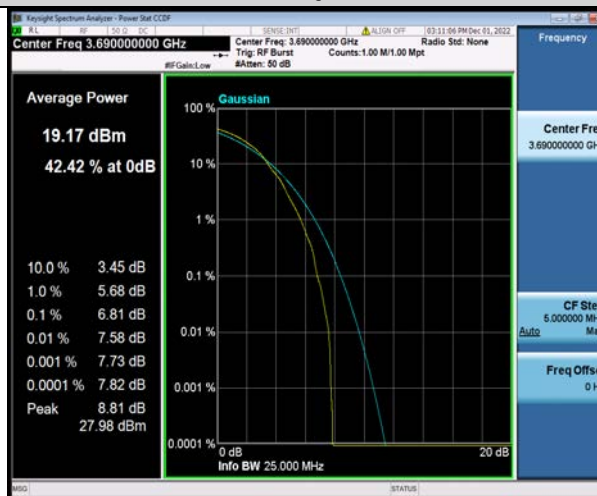
Band48-20MHz-64QAM-56640-100RB#0
