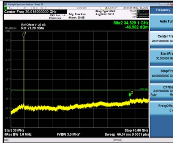
Band48-10MHz-64QAM-55290-1RB#0-Range1:30~40000MHz
