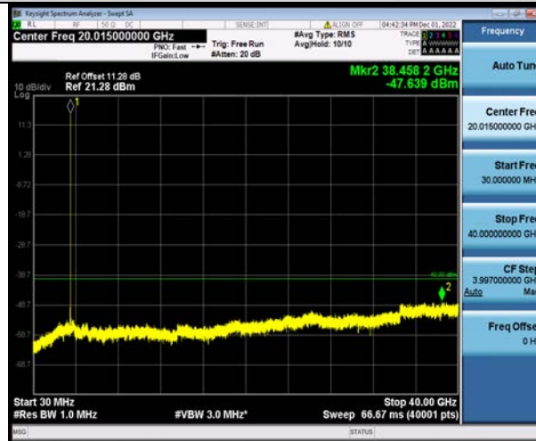
Band48-10MHz-QPSK-55990-1RB#0-Range1:30~40000MHz
