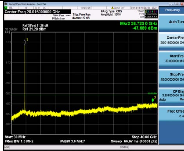
Band48-15MHz-QPSK-55315-1RB#0-Range1:30~40000MHz
