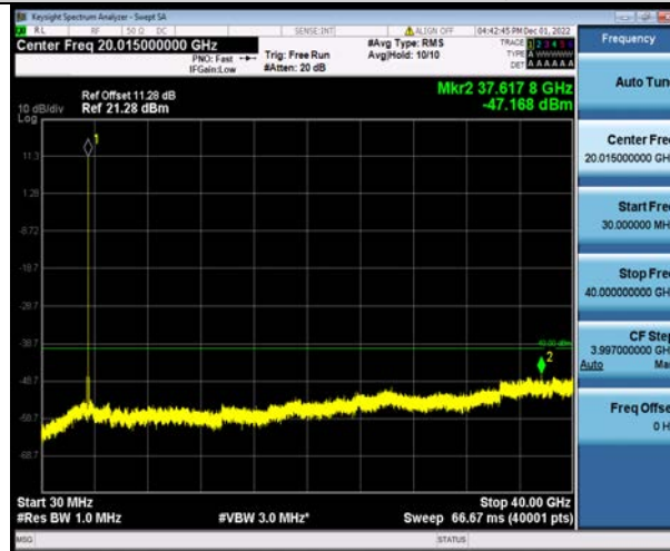
Band48-10MHz-16QAM-55990-1RB#0-Range1:30~40000MHz
