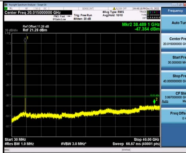
Band48-20MHz-64QAM-55340-1RB#0-Range1:30~40000MHz
