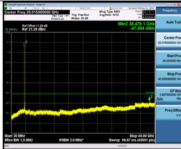
Band48-15MHz-64QAM-55315-1RB#0-Range1:30~40000MHz
