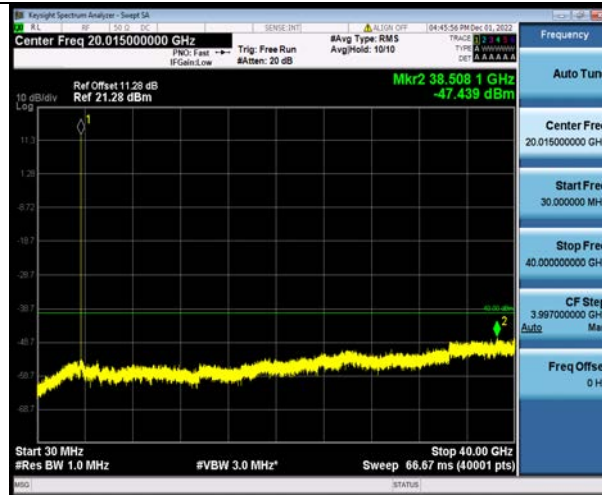
Band48-15MHz-16QAM-55315-1RB#0-Range1:30~40000MHz
