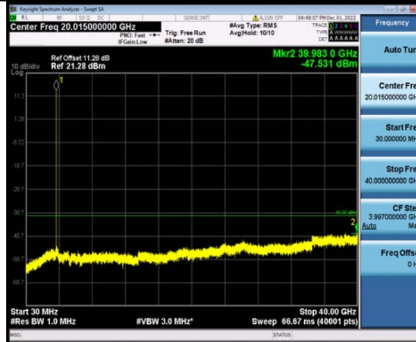
Band48-20MHz-16QAM-55340-1RB#0-Range1:30~40000MHz
