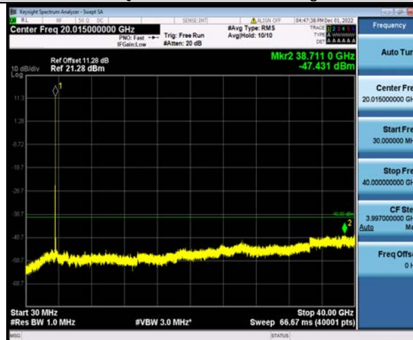
Band48-20MHz-16QAM-56640-1RB#0-Range1:30~40000MHz
