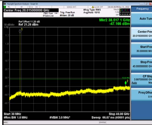
Band48-15MHz-16QAM-55990-1RB#0-Range1:30~40000MHz
