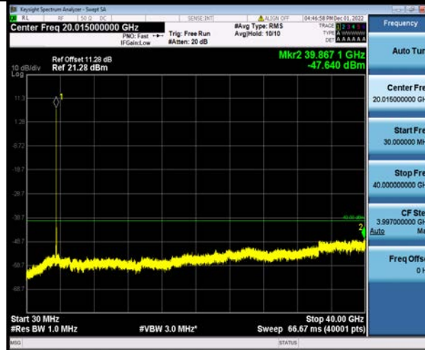
Band48-20MHz-16QAM-55990-1RB#0-Range1:30~40000MHz
