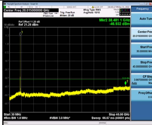
Band48-15MHz-QPSK-56665-1RB#0-Range1:30~40000MHz
