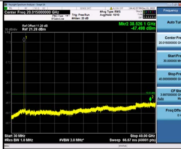
Band48-10MHz-64QAM-55990-1RB#0-Range1:30~40000MHz
