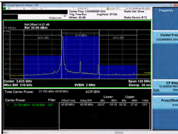
N48-40MHz-QPSK-641666-1RB#104
