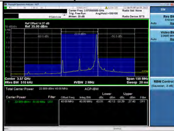
N48-40MHz-QPSK-638000-100RB#0
