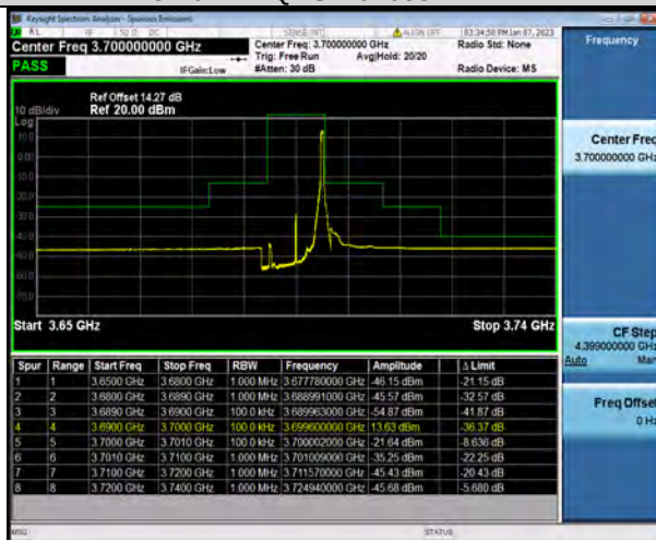
N48-10MHz-QPSK-646332-25RB#0
