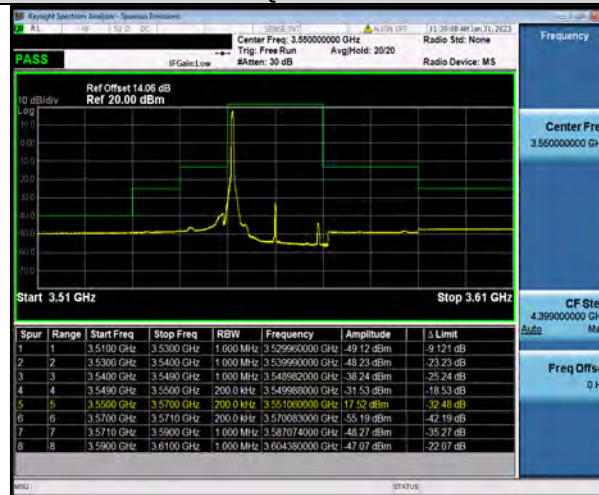
N48-20MHz-QPSK-637334-1RB#50
