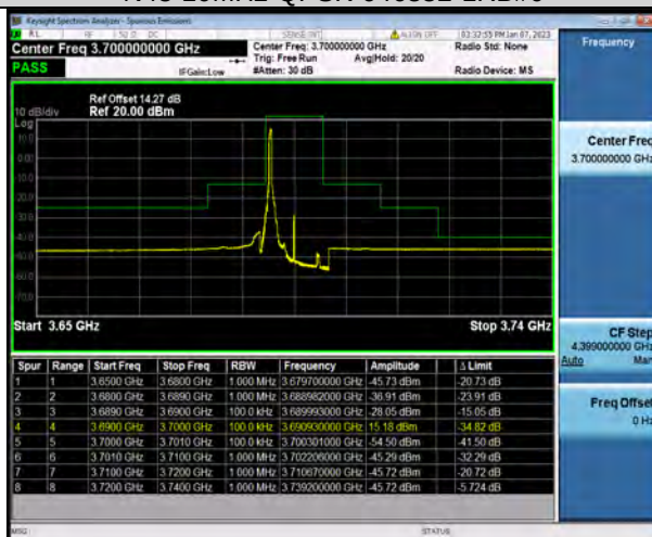
N48-10MHz-QPSK-646332-1RB#24
