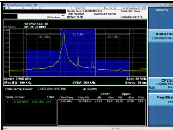
N48-10MHz-QPSK-646332-1RB#24
