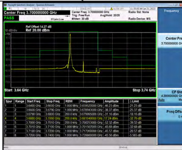
N48-20MHz-QPSK-646000-1RB#50
