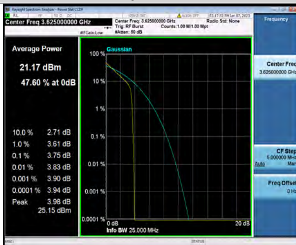
N48-20MHz-QPSK-637334-50RB#0
