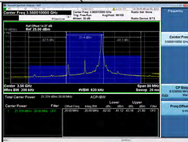
N48-20MHz-QPSK-637334-50RB#0
