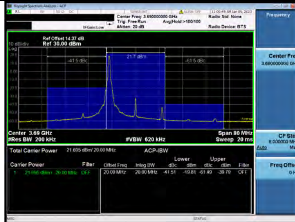
N48-20MHz-QPSK-646000-1RB#50
