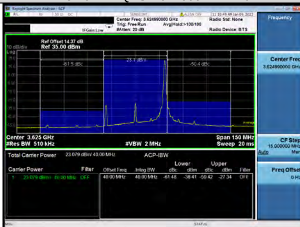
N48-40MHz-QPSK-641666-100RB#0
