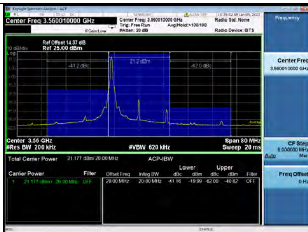
N48-20MHz-QPSK-637334-1RB#50
