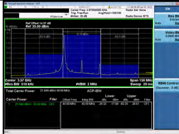
N48-40MHz-QPSK-638000-1RB#104
