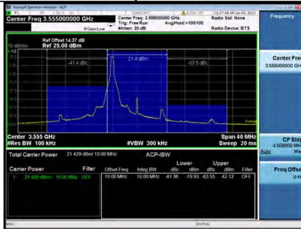
N48-10MHz-QPSK-637000-1RB#24
