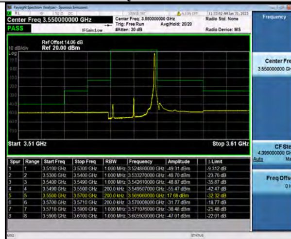
N48-20MHz-QPSK-637334-50RB#0
