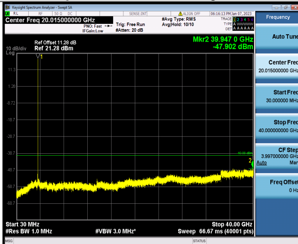
N48-10MHz-QPSK-646332-1RB#0-Range1:30~40000MHz
