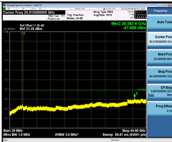
N48-20MHz-QPSK-637334-1RB#0-Range1:30~40000MHz
