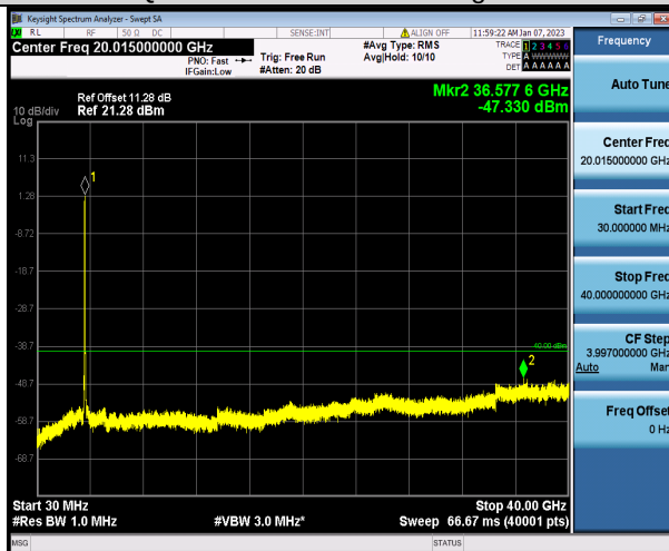
N48-40MHz-QPSK-645332-1RB#0-Range1:30~40000MHz
