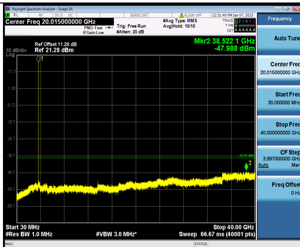
N48-40MHz-QPSK-638000-1RB#0-Range1:30~40000MHz
