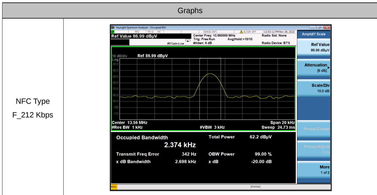
20dB Bandwidth & 99% Bandwidth Plot
