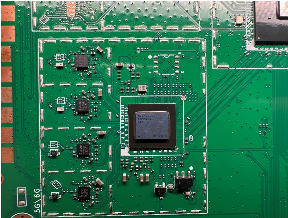
(11) EUT Photo Wi-Fi Chip
