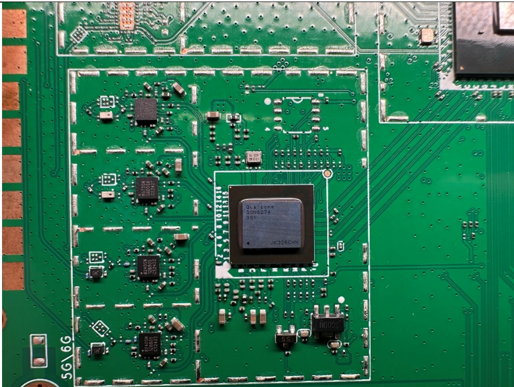
(10) EUT Photo Wi-Fi Chip
