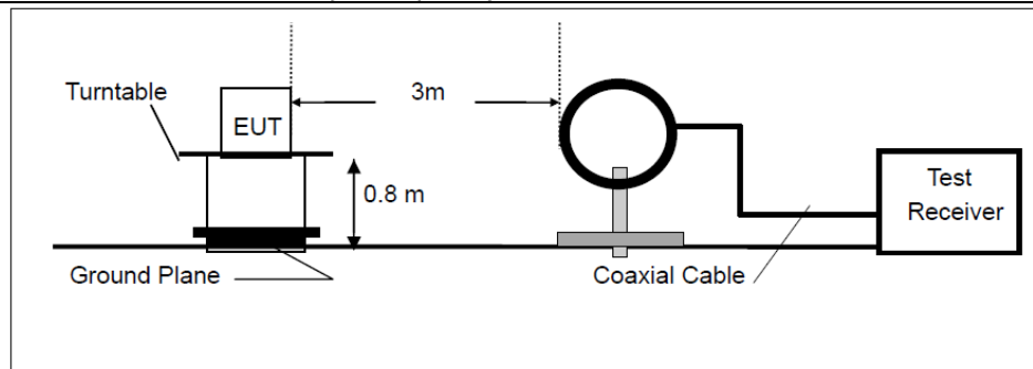
2. Radiated Emission Test Set-Up, Frequency Below 1000 MHz
