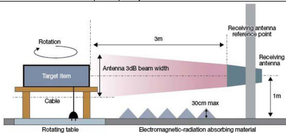
3. Radiated Emission Test Set-Up, Frequency above 1000MHz
