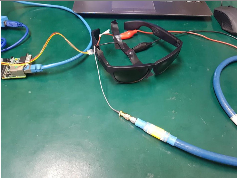
Conducted (2)
