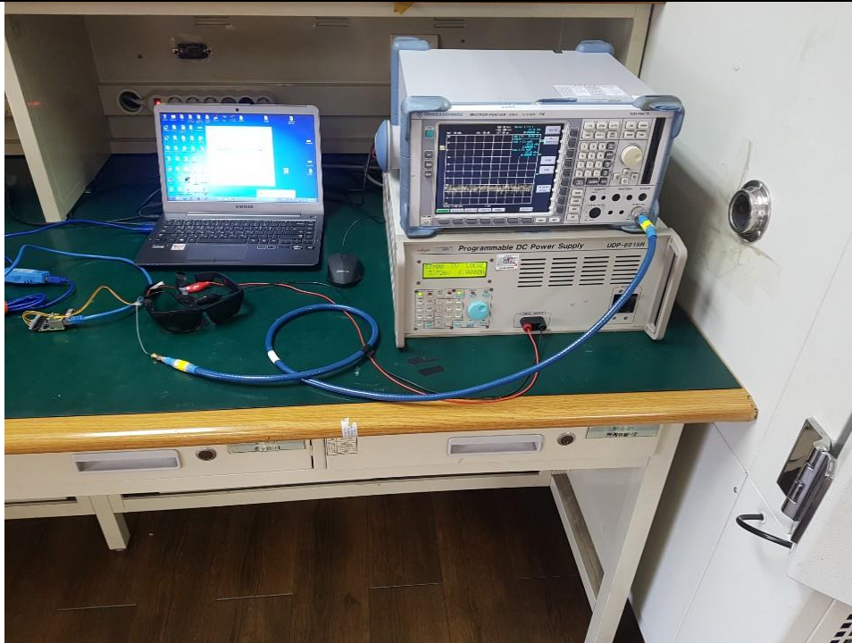
Conducted (1)
