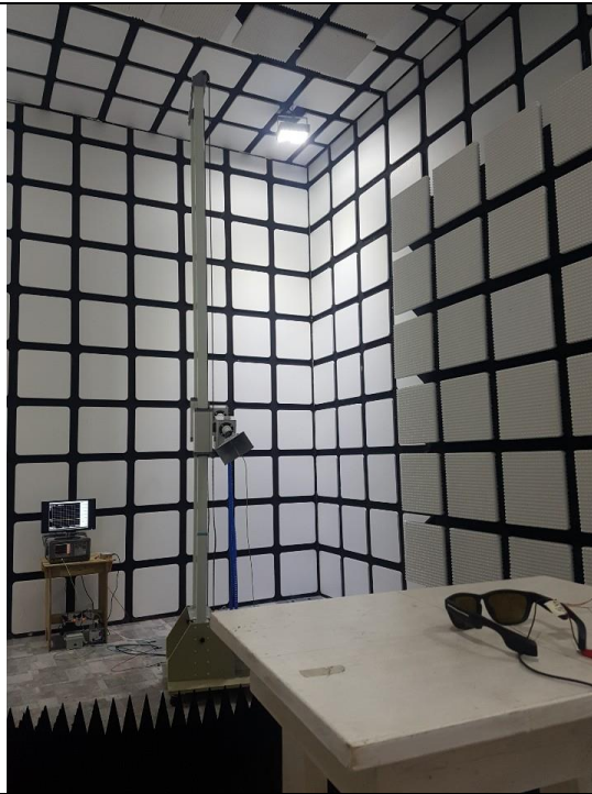
Above 1 GHz
