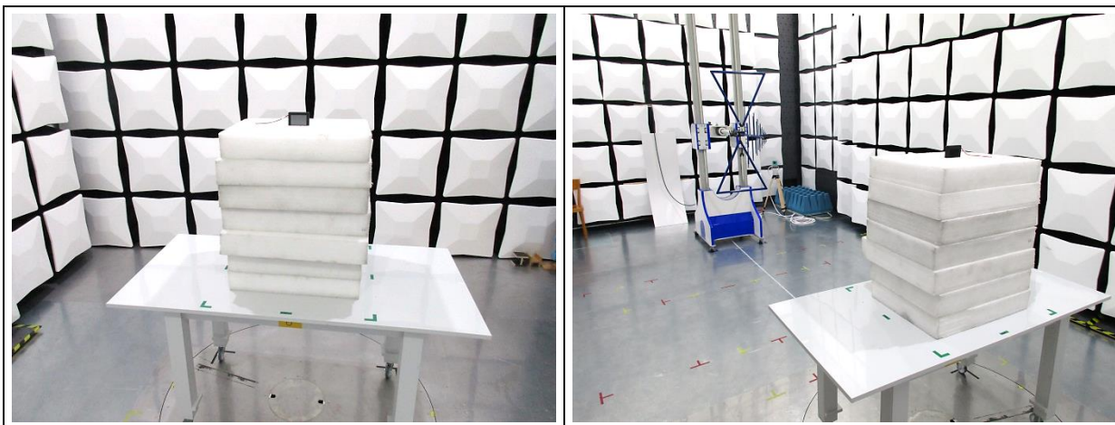
Fig 2 Radiated measurements – Carrier EIRP and antenna gain (radiated)
