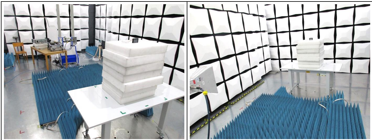
Fig 5 Spurious emissions 1 GHz – 9.3 GHz
