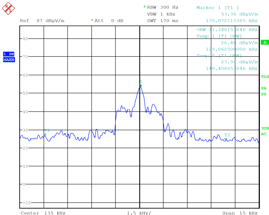
Occupied Bandwidth @ 99%
