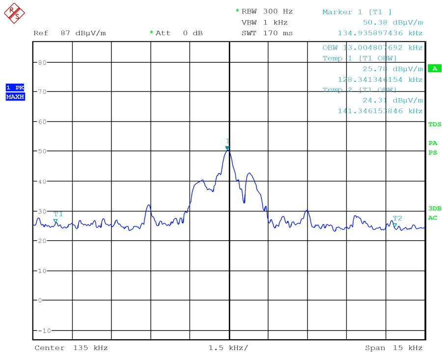
Occupied Bandwidth @ 99%
