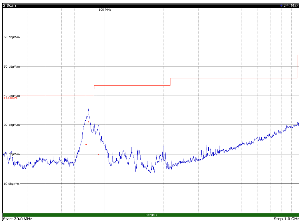
Horizontal polarization
