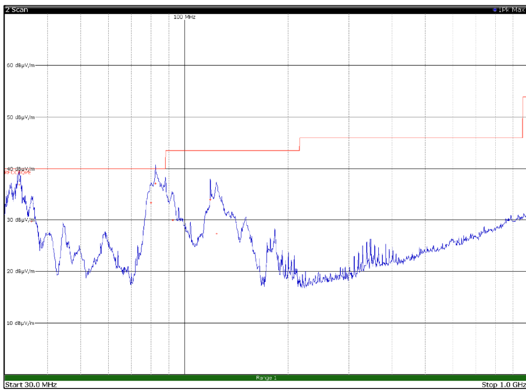
Vertical polarization
