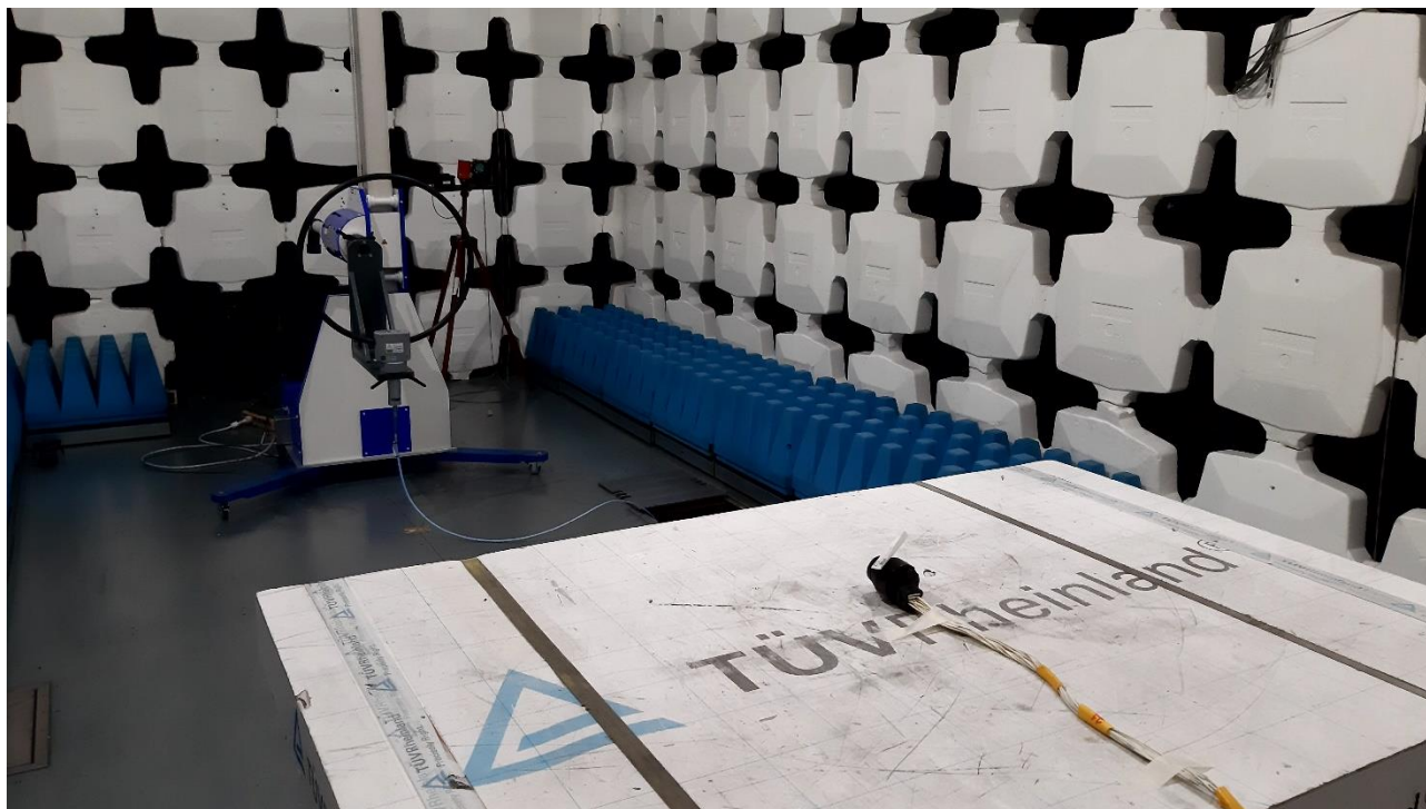
radiated emission test set-up (range 0.15-30MHz)
