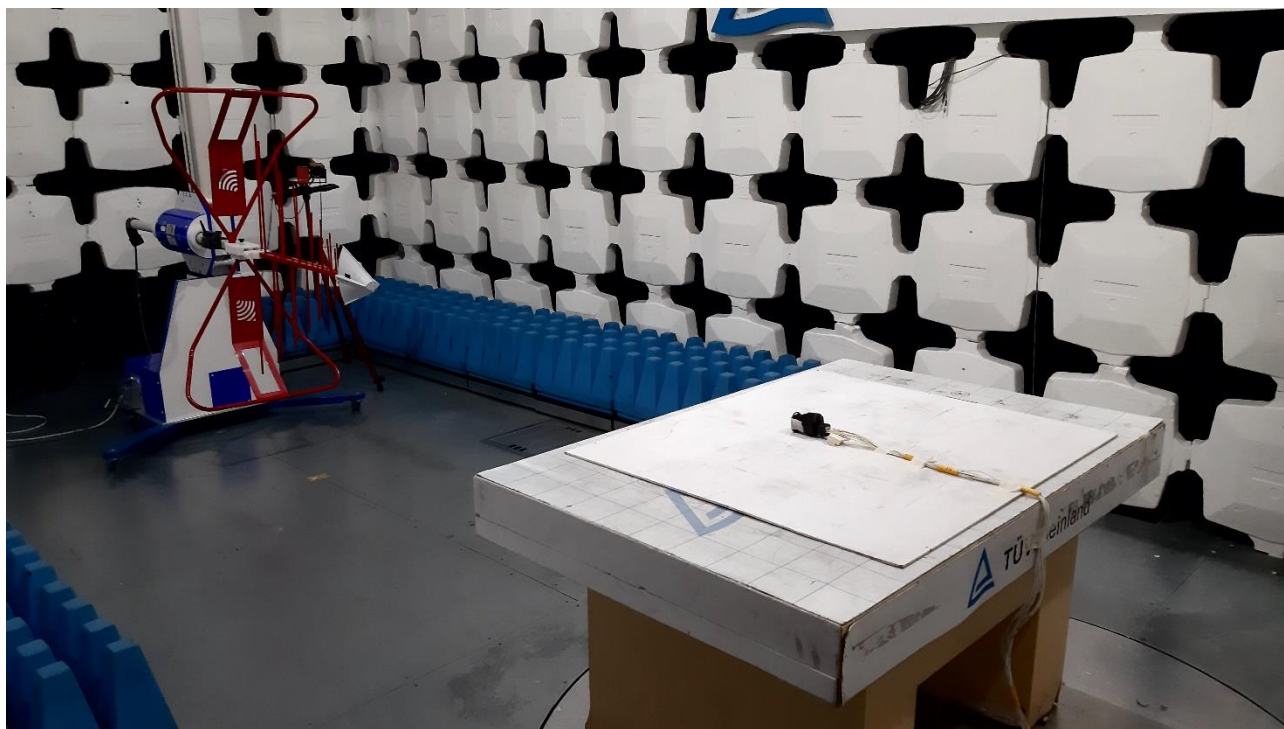
radiated emission test set-up (range 30-1000MHz)
