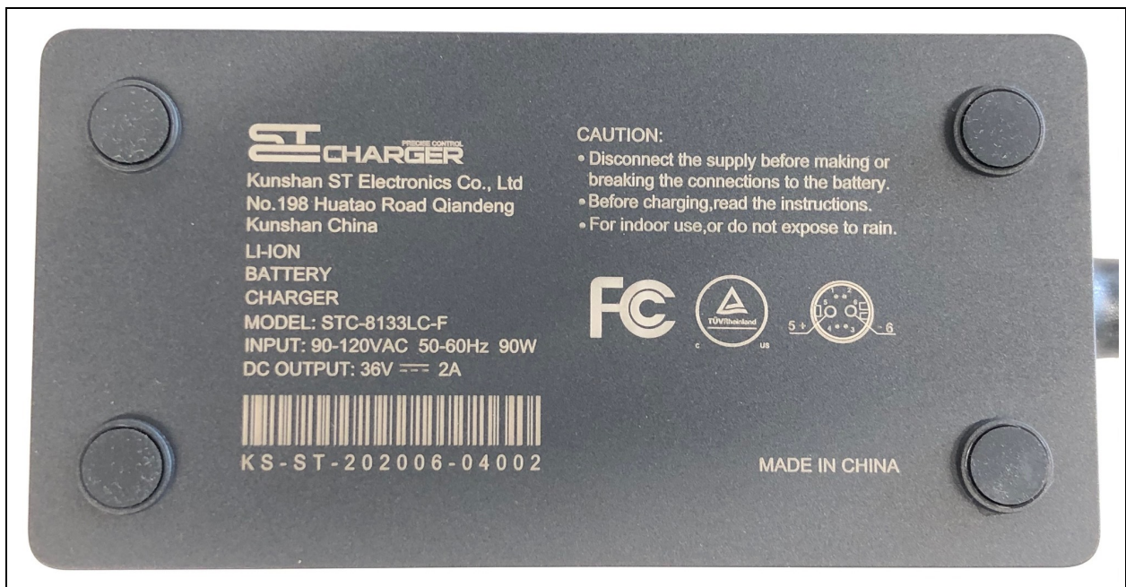
Figure 4-5: Copy of type plate of the charger STC-8133LC-F (Serial production)
