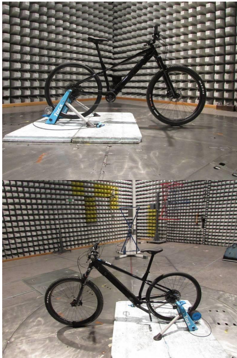
Figure 6-2: test setup for Radiated disturbances 30 MHz to 1000 MHz
