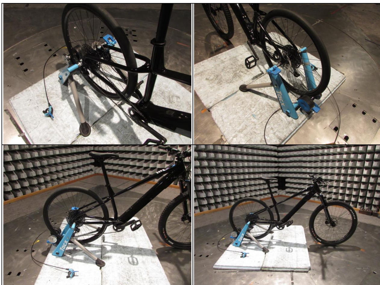
Figure 4-12: EPAC in the training bike stand (Tacx)
