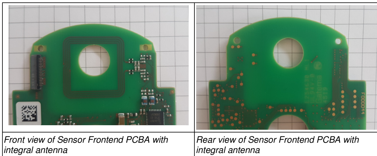
Figure 2: Sensor Frontend PCBA (F000044) – Antenna
