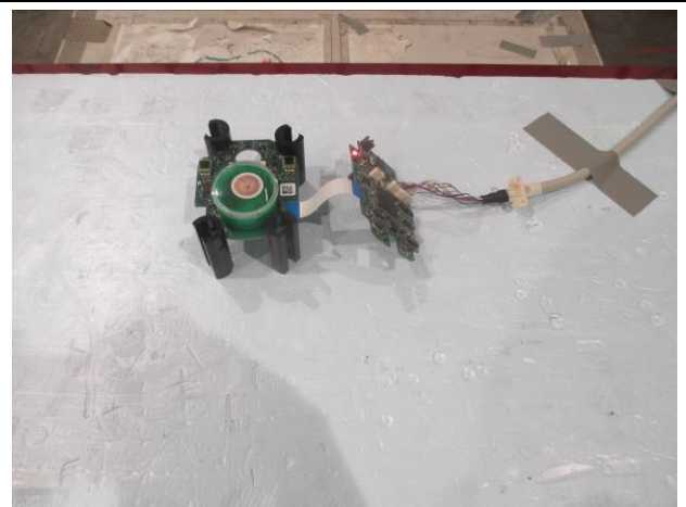
Figure 7-24: Test Setup Radiated Emission 9 kHz – 30 MHz – Configuration 1, 2, 3, 4
