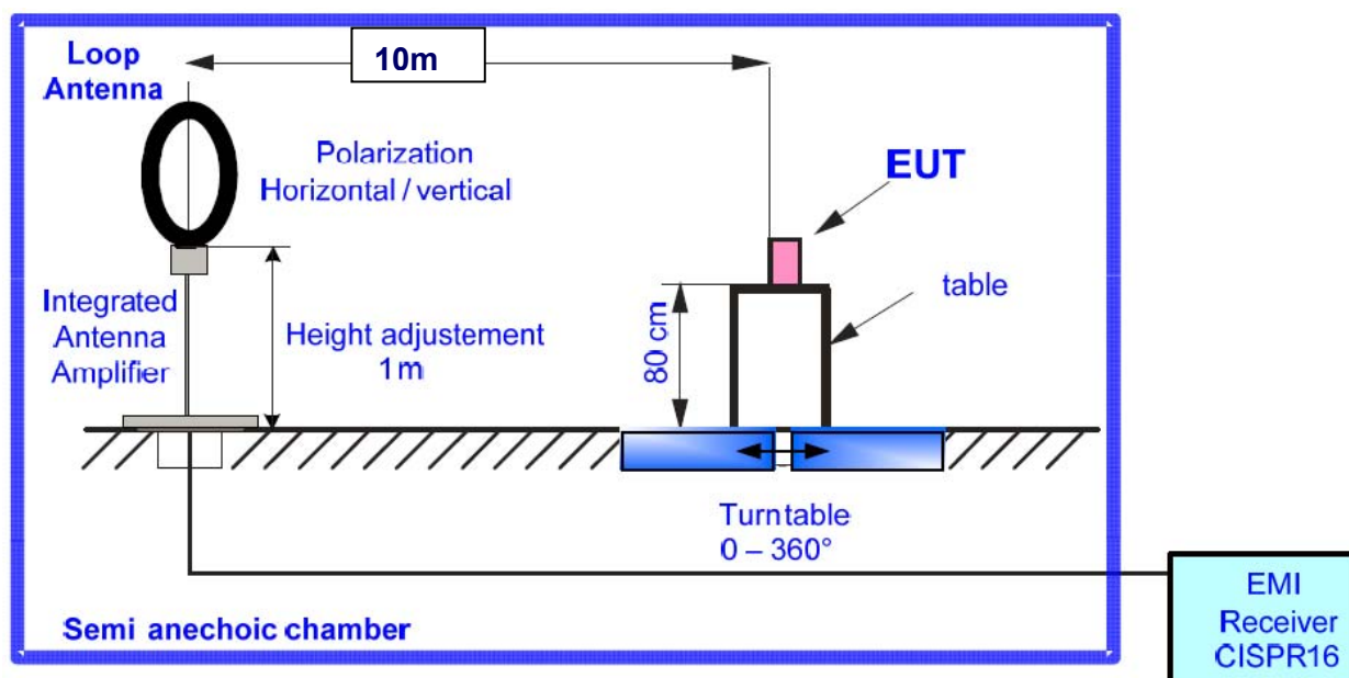
Figure 6-4: test setup for Radiated disturbances 9 kHz to 30 MHz
