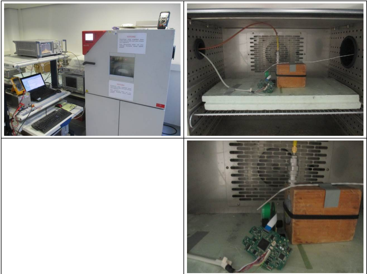
Figure 7-25: Test Setup – Frequency Stability with voltage or/and Temperature variation – Configuration 2
