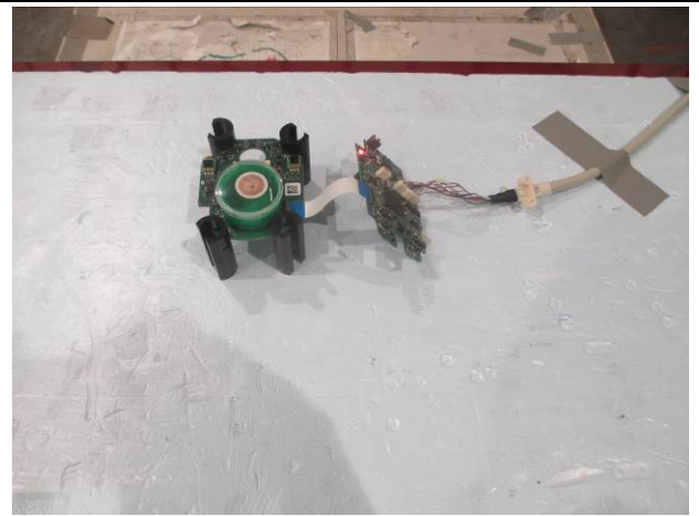
Figure 4: Test Setup Radiated Emission 9 kHz – 30 MHz – Configuration 1, 2, 3, 4
