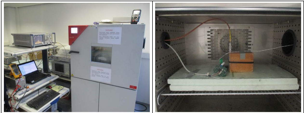
Figure 2: Test Setup Occupied Bandwidth – Configuration 2
