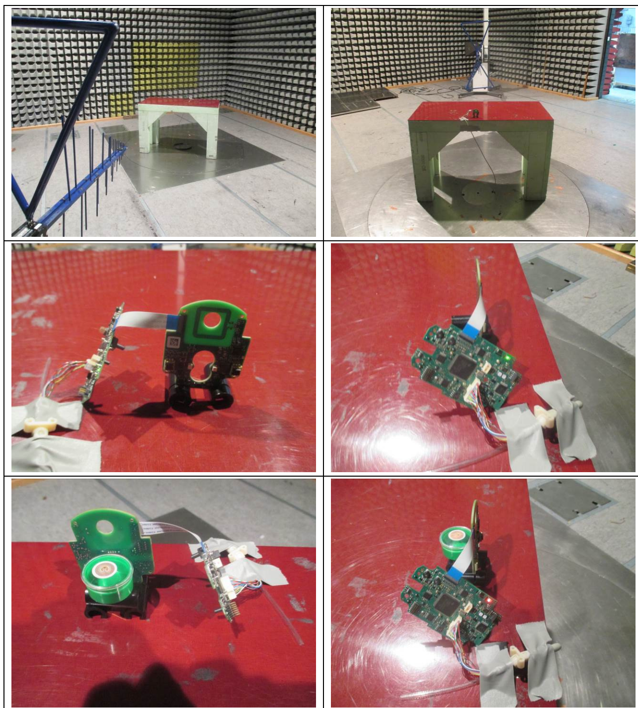
Figure 3: Test Setup Radiated Emission 30 MHz – 1 GHz – Configurations 1, 2
