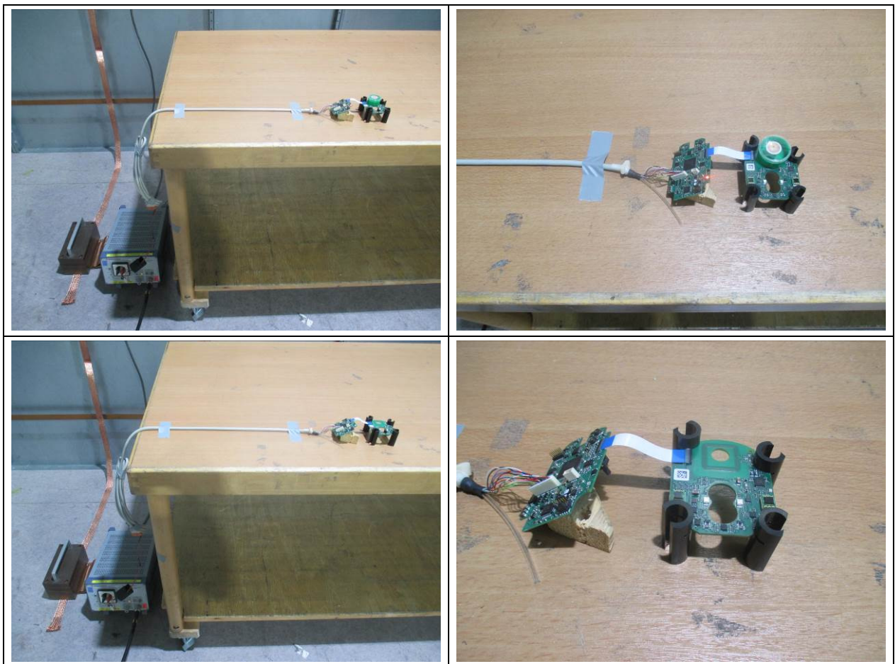
Figure 1: Test Setup Conducted Emissions (150 kHz – 30 MHz) – Configurations 3, 4, 5
