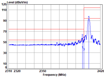
Headset 2.4G SRD_TX_CH_L_Horizontal
