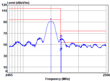
Headset 2.4G SRD_TX_CH_H_Horizontal
