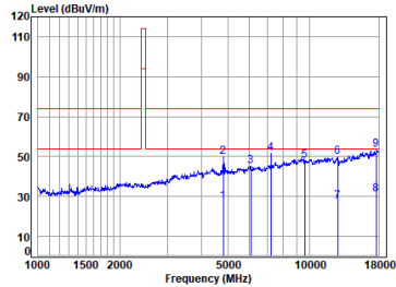
Headset 2.4G SRD_TX_CH_L_Horizontal
