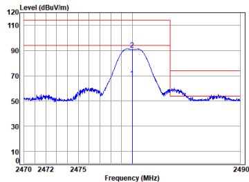
Headset 2.4G SRD_TX_CH_H_Horizontal
