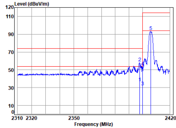
Headset 2.4G SRD_TX_CH_L_Vertical
