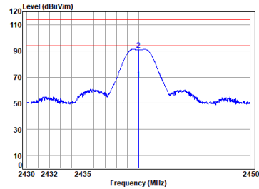
Headset 2.4G SRD_TX_CH_M_Vertical
