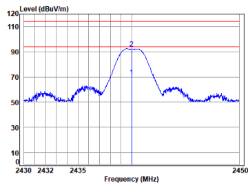
Headset 2.4G SRD_TX_CH_M_Horizontal
