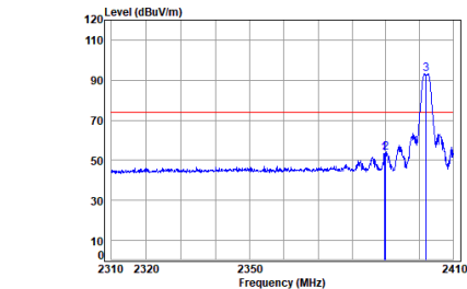
BLE_2M_TX_CH_00_Vertical-Peak
