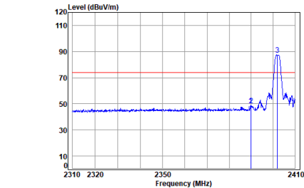
BLE_2M_TX_CH_00_Horizontal-Peak
