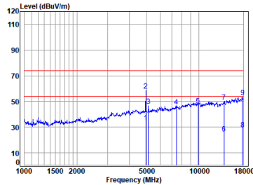
Headset BT_DH5_TX_CH_78_Horizontal
