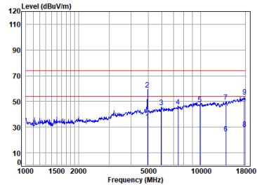
Headset BT_DH5_TX_CH_78_Vertical
