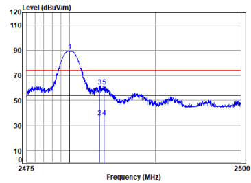
Headset BT_DH5_TX_CH_78_Vertical
