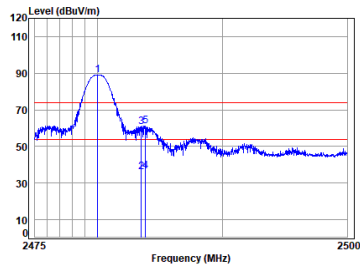
Headset BT_DH5_TX_CH_78_Horizontal
