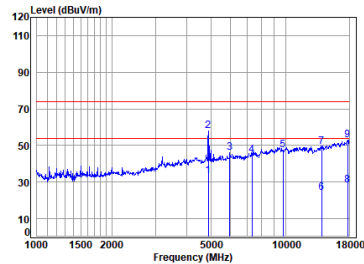
Headset BT_DH5_TX_CH_39_Vertical
