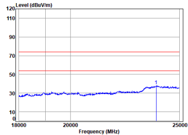
BT_TX_CH_00_Vertical
