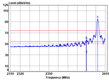
Headset BT_DH5_TX_CH_00_Horizontal
