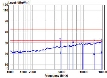
Headset BT_DH5_TX_CH_00_Horizontal
