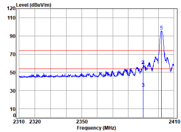
Headset BT_DH5_TX_CH_00_Vertical
