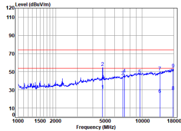
Headset BT_DH5_TX_CH_00_Vertical
