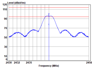
Dongle 2.4G SRD_TX_CH_M_Horizontal
