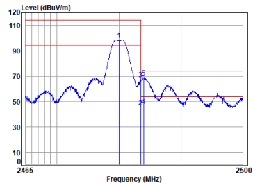
Dongle 2.4G SRD_TX_CH_H_Vertical
