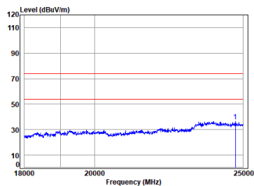
Dongle 2.4G SRD_TX_CH_M_Horizontal
