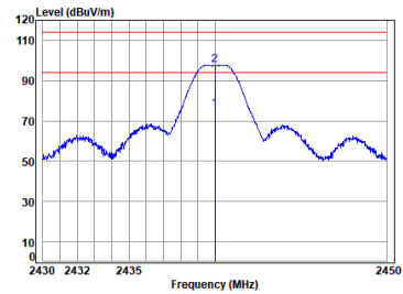
Dongle 2.4G SRD_TX_CH_M_Vertical
