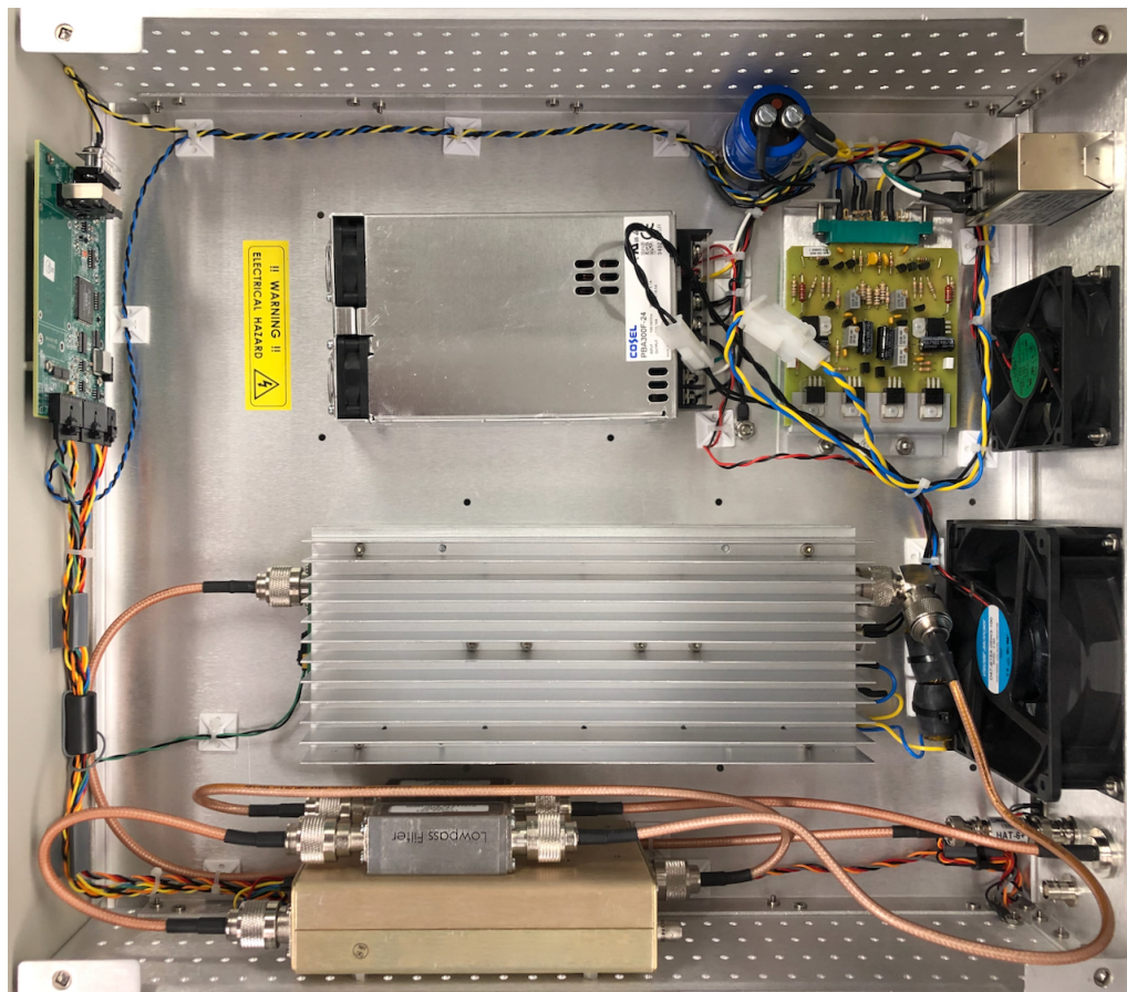
Assembled Transmit Chassis without amplifier hood
