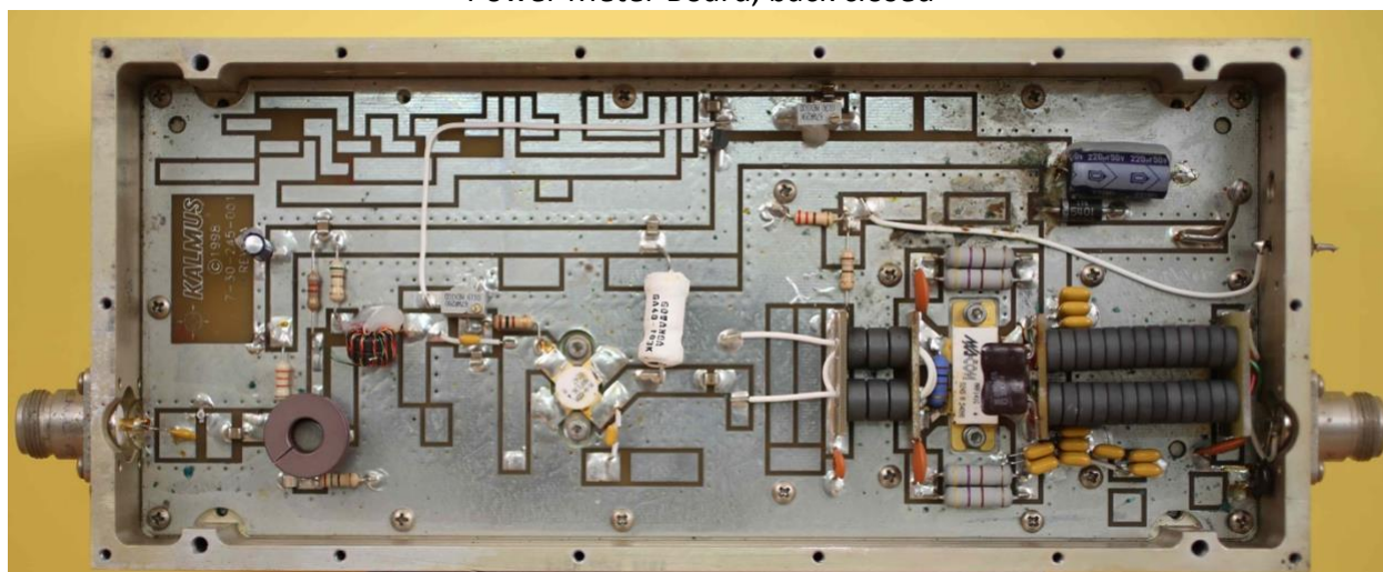
Power Amplifier, front open, no component on back side
