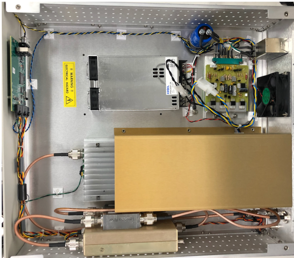
Assembled Transmit Chassis with amplifier hood
