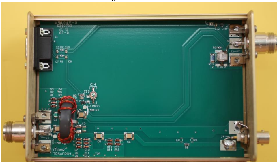
Power Meter Board, front open
