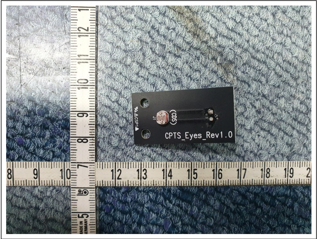
SubBoard-Rear
