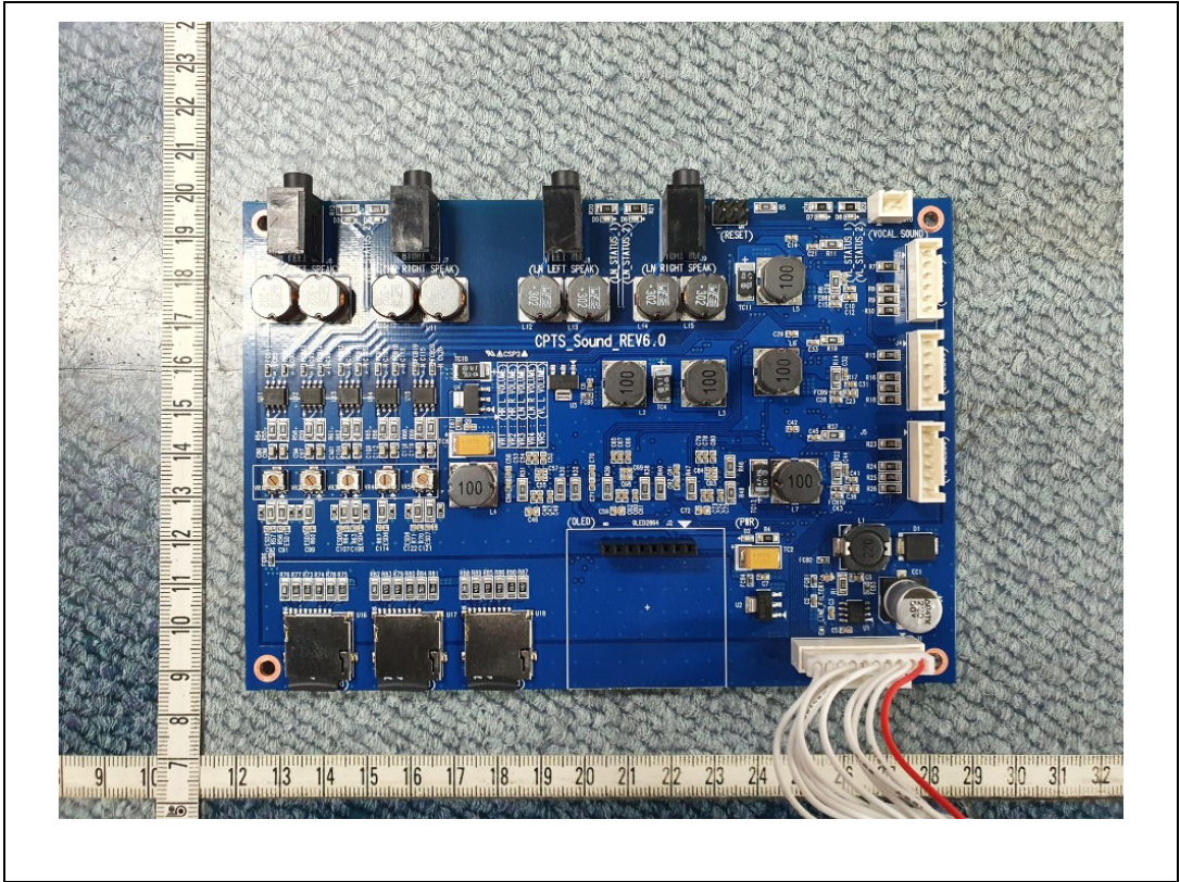
MainBoard-Rear
