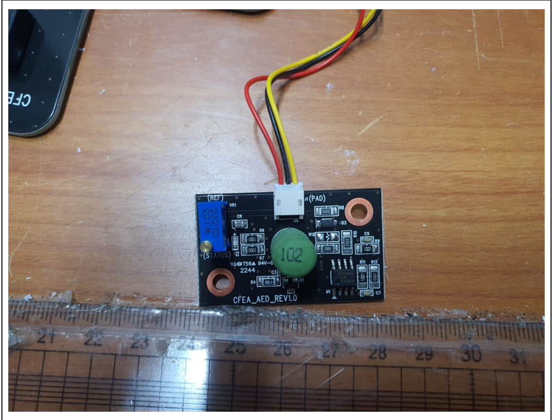
Board-Rear
