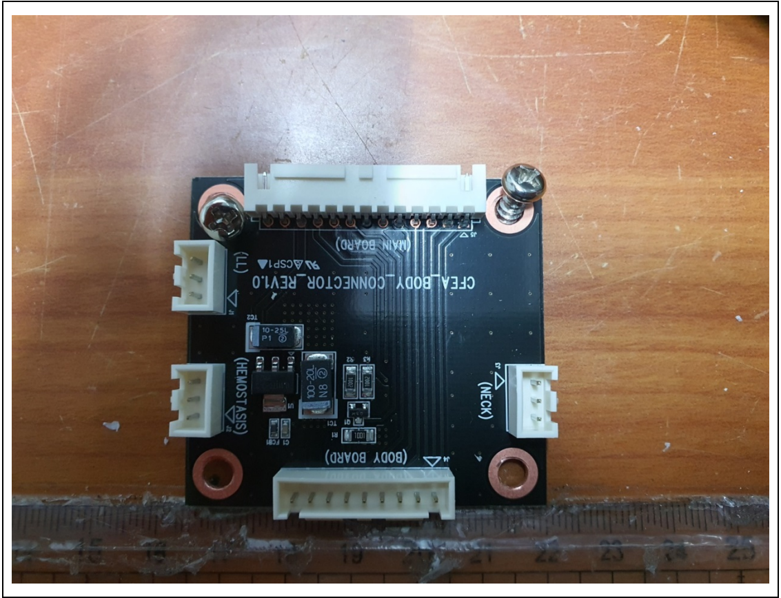
Board-Front
