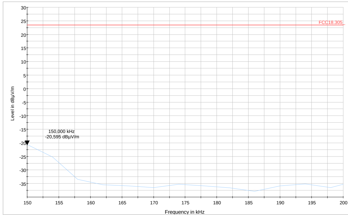
Diagram 5: EUT lying
