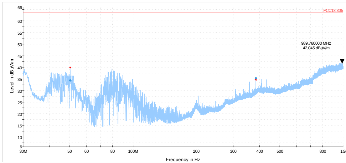
Diagram 10: Op. Mode 1, EUT is at standing position
