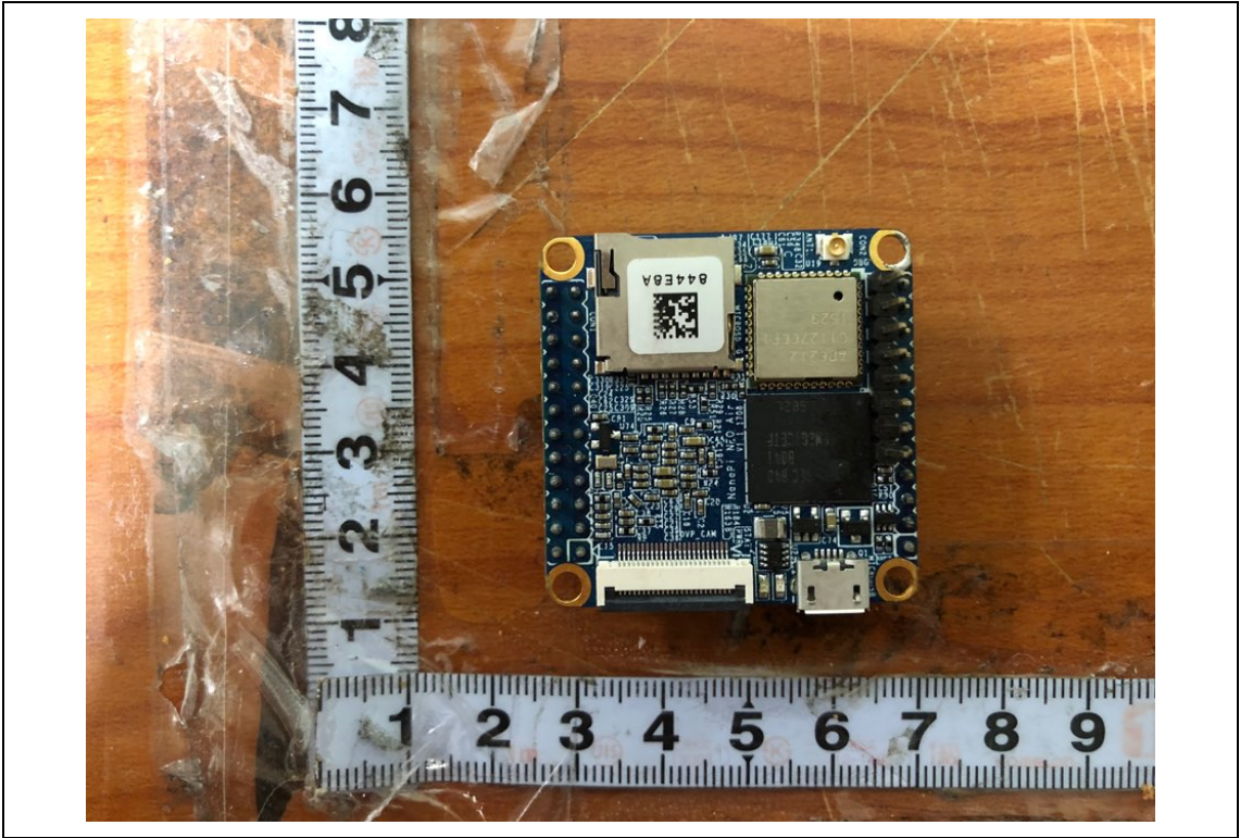
Module Board–Rear
