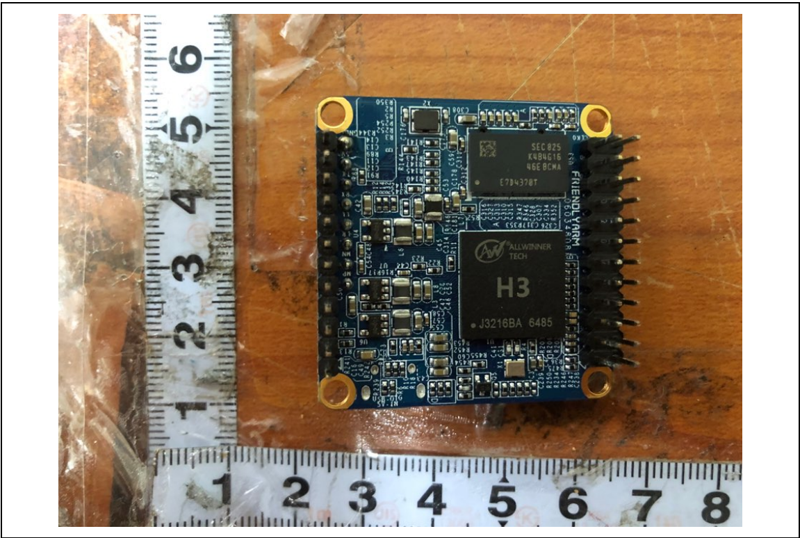
Module Board–Rear
