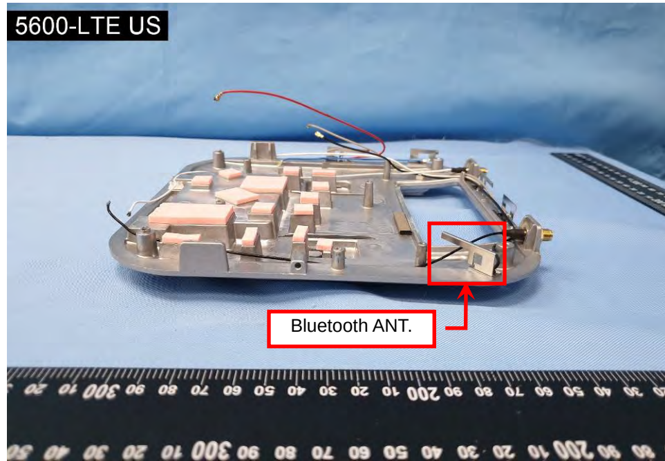
EUT Photo (45)
