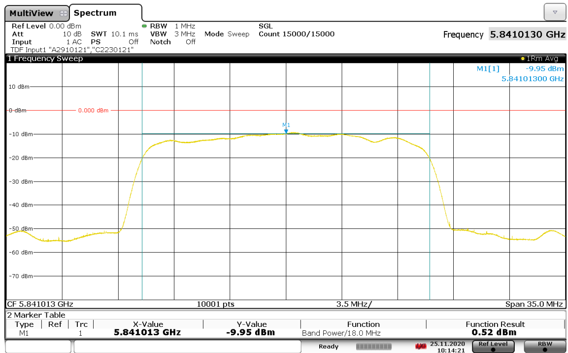
Graph 6-10: Measured Conducted Power, High Channel
