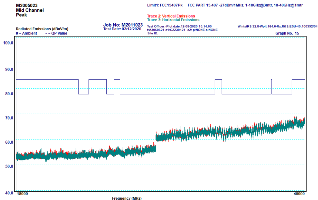
Graph 6-29: Transmitter Spurious Emissions, 18 – 40 GHz, Mid Channel, Peak
