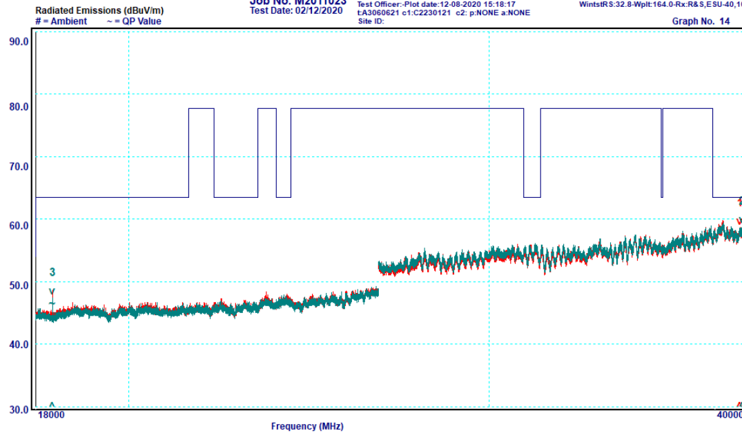
Graph 6-31: Transmitter Spurious Emissions, 18 – 40 GHz, Low Channel, Average
