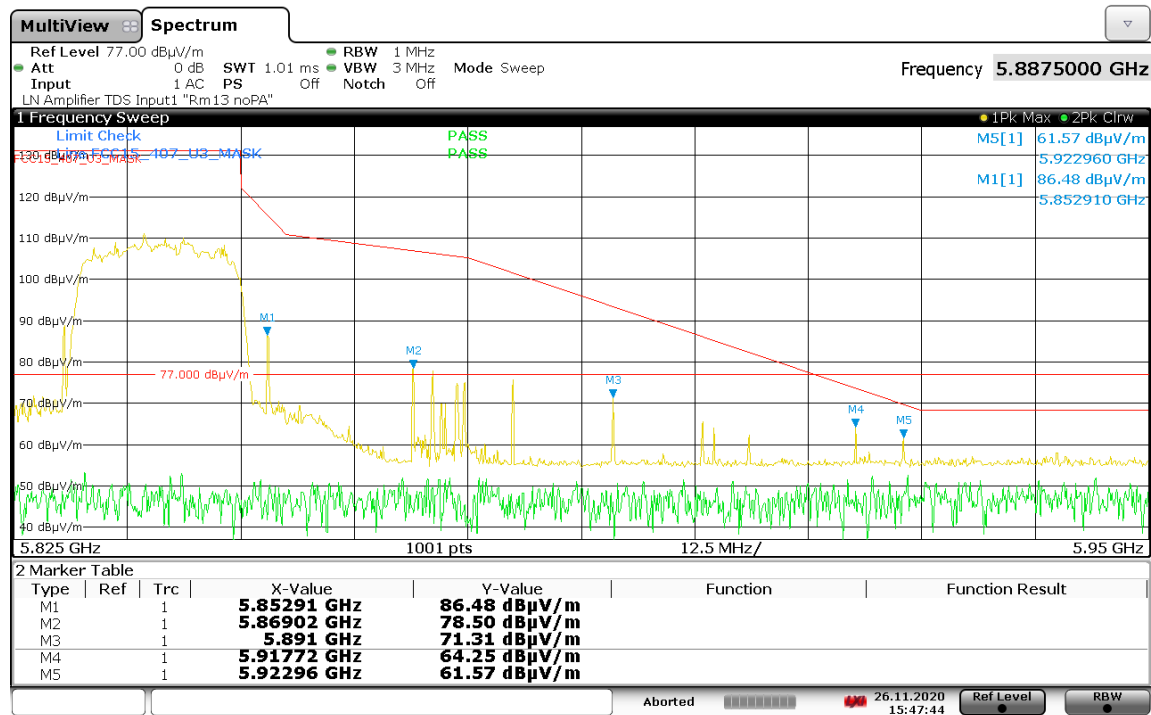
Graph 6-15: Band-Edge Emission, Upper edge
