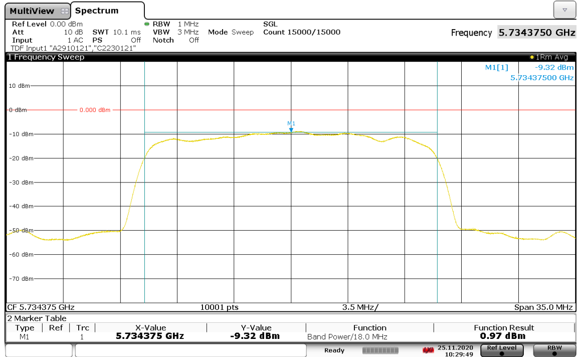
Graph 6-8: Measured Conducted Power, Low Channel
