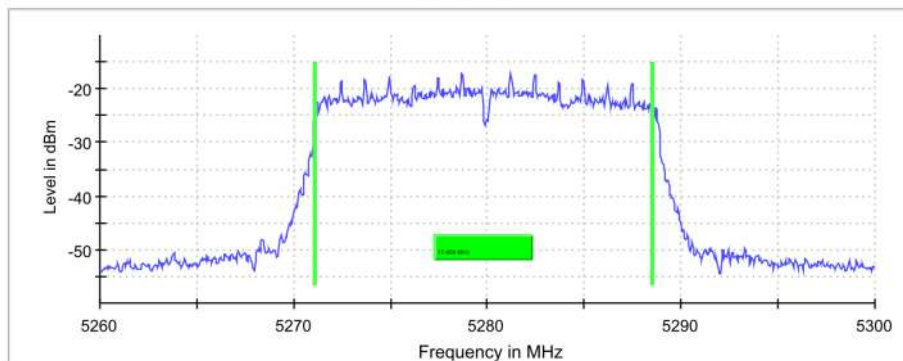
6 dB Bandwidth
