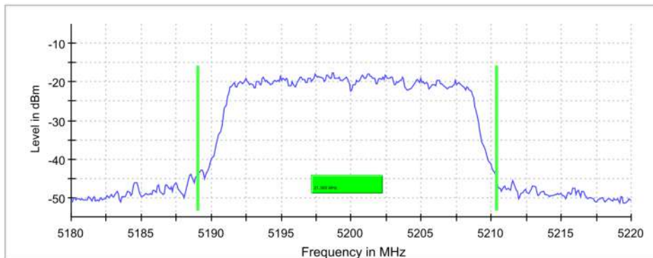
26 dB Bandwidth
