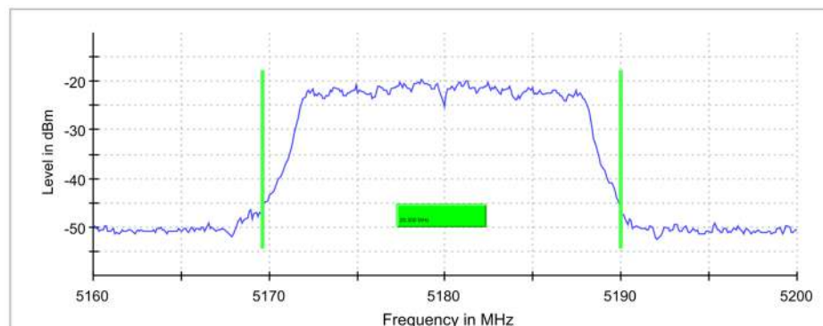
26 dB Bandwidth
