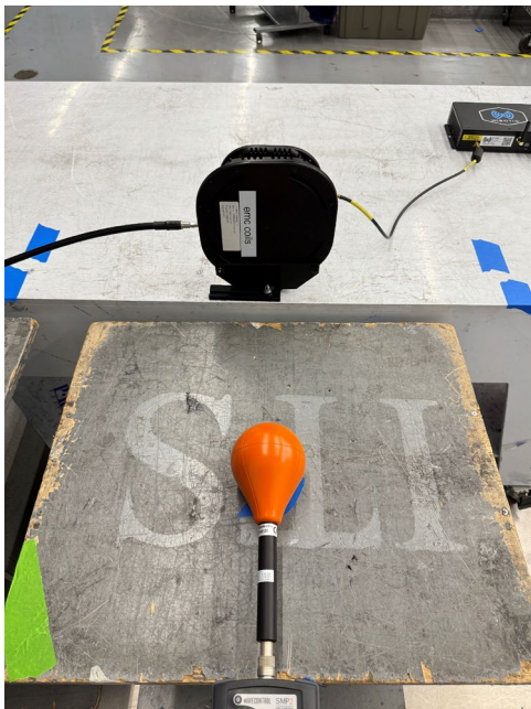
Transmitter Front
