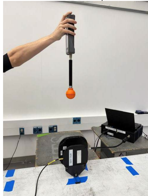
Transmitter Top
