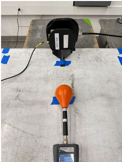
Receiver Front
