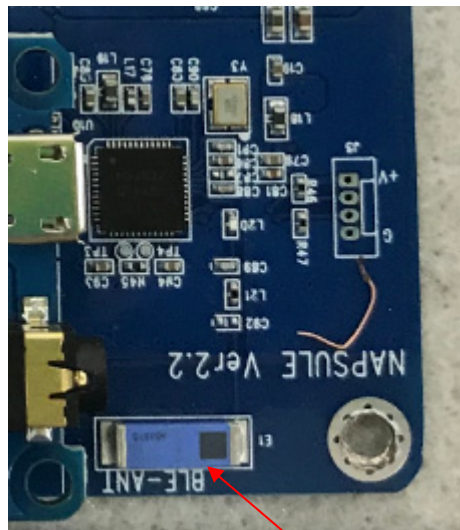
Chip Antenna (Bluetooth LE)
