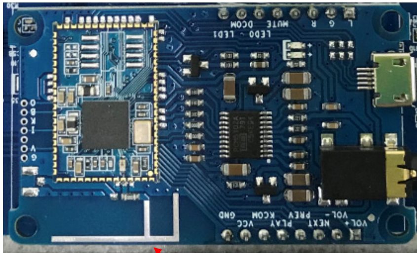
PCB Pattern Antenna (Bluetooth)
