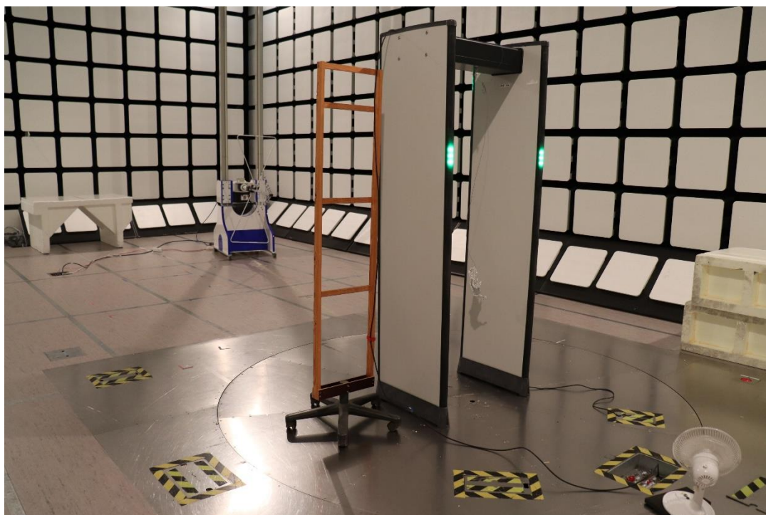
Photograph 3. Radiated Emissions 30 MHz – 1000 MHz
