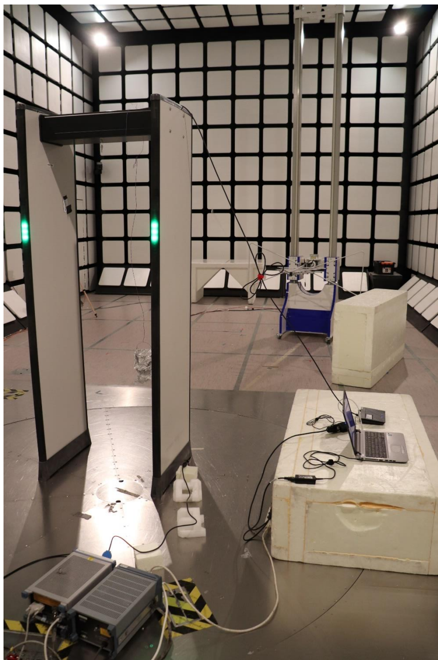
Photograph 1. Conducted Emissions test set-up
