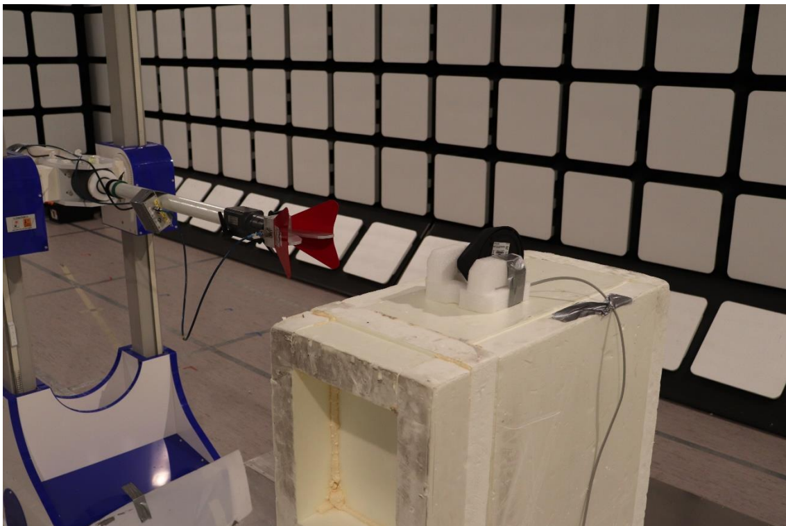
Photograph 8. Radiated Emissions 1 – 1.61 GHz and 10.6 – 18 GHz
