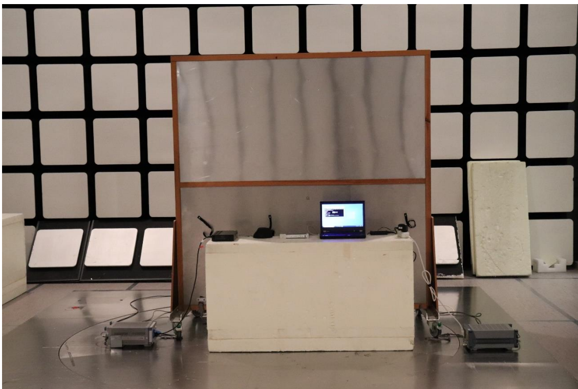
Photograph 12. Conducted Emission
