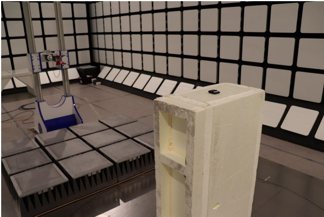
Photograph 9. Radiated Emissions 1.61 – 10.6 GHz
