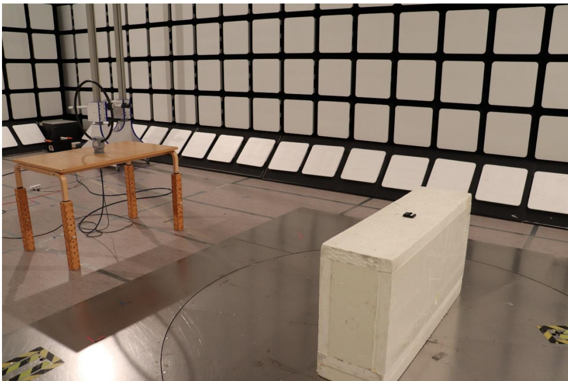
Photograph 6. Radiated Emissions 9kHz – 30 MHz
