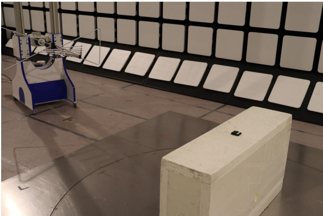
Photograph 7. Radiated Emissions 30 – 1000 MHz
