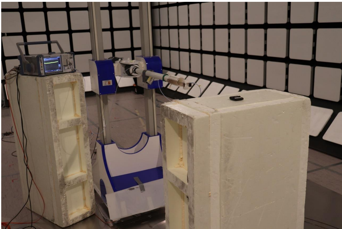
Photograph 11. Radiated Emission 26.5 – 40 GHz
