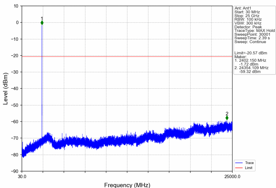
8DPSK 3DH5 LCH_2402MHz_Ant1_NTNV
