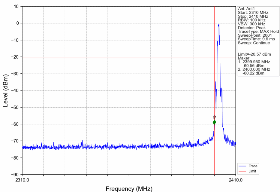
8DPSK 3DH5 LCH_2402MHz_Ant1_NTNV
